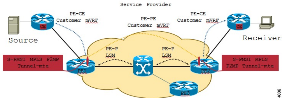
Figure 7: Multicast VRF
