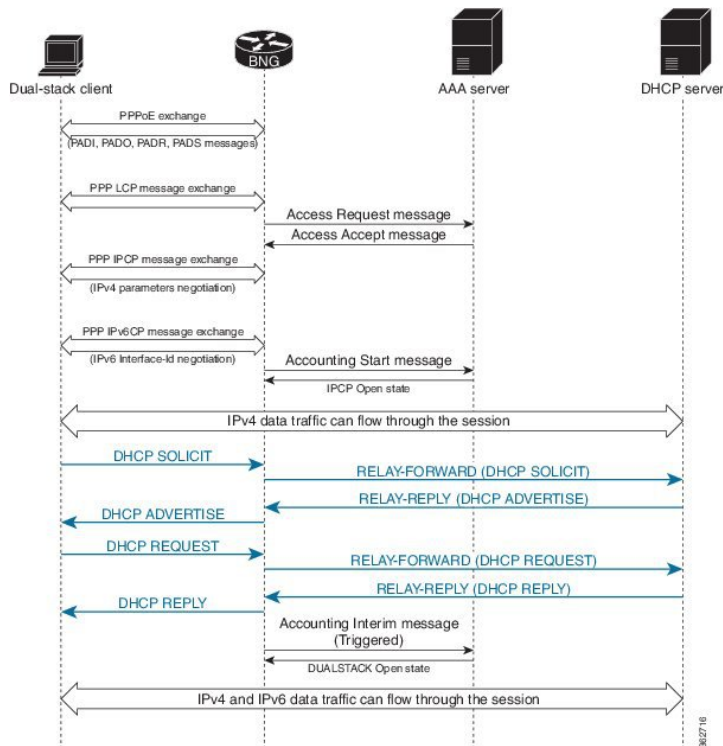
Figure 57: Call Flow of PPPoE Dual-Stack - DHCPv6-Based Address Assignment
