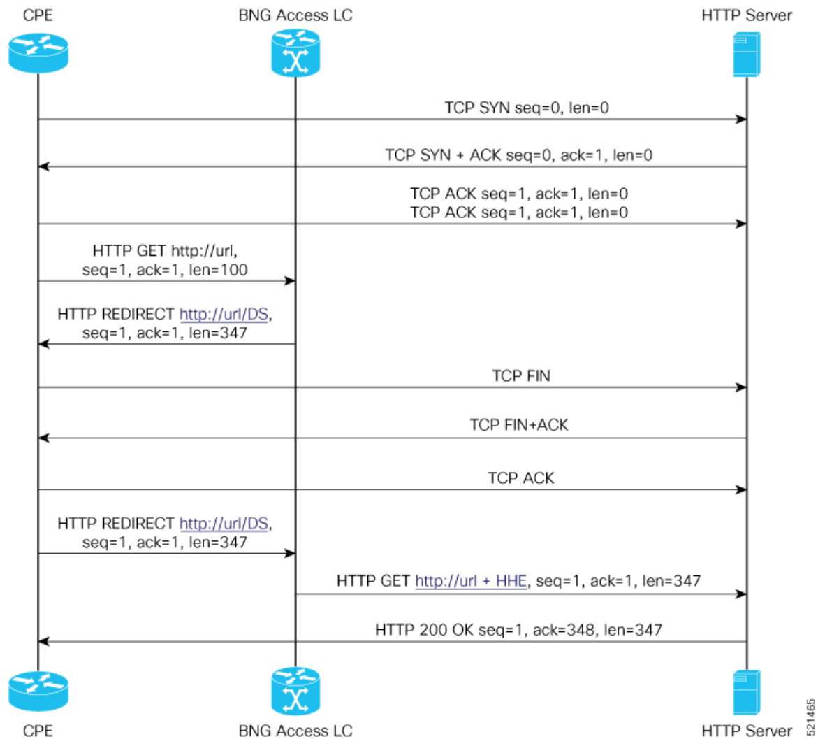
Figure 27: Sequence of events for HTTP Header Enrichment
