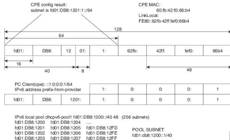
Figure 52: Sample IPv6 Address Mapping for Dual-Stack Subscriber
