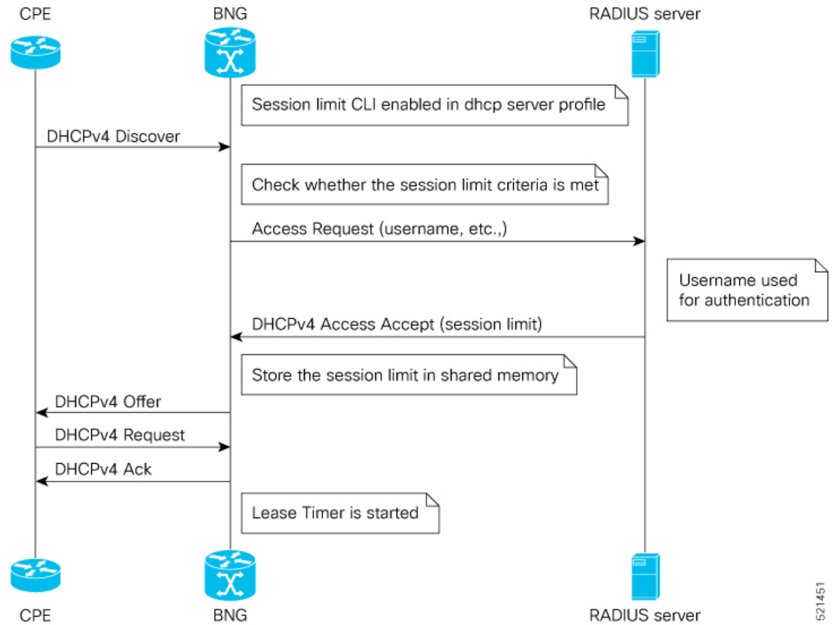
Figure 22: Sequence of events for limiting DHCPv4 sessions
