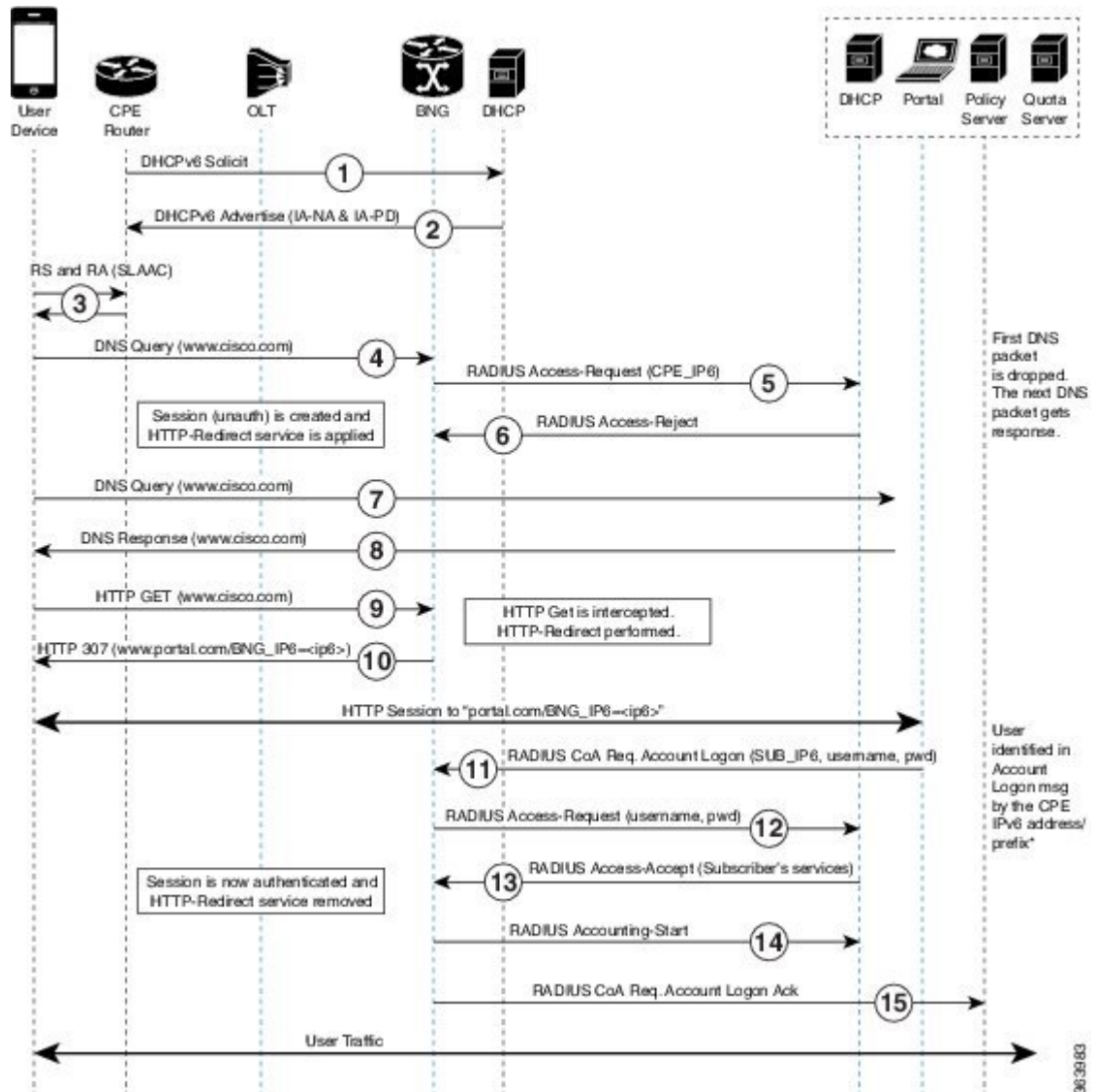
Figure 12: Call Flow of Web-Login IPv6 Routed Subscriber Session
