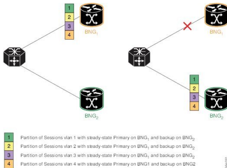
Figure 30: Active-standby Mode of Session Distribution
