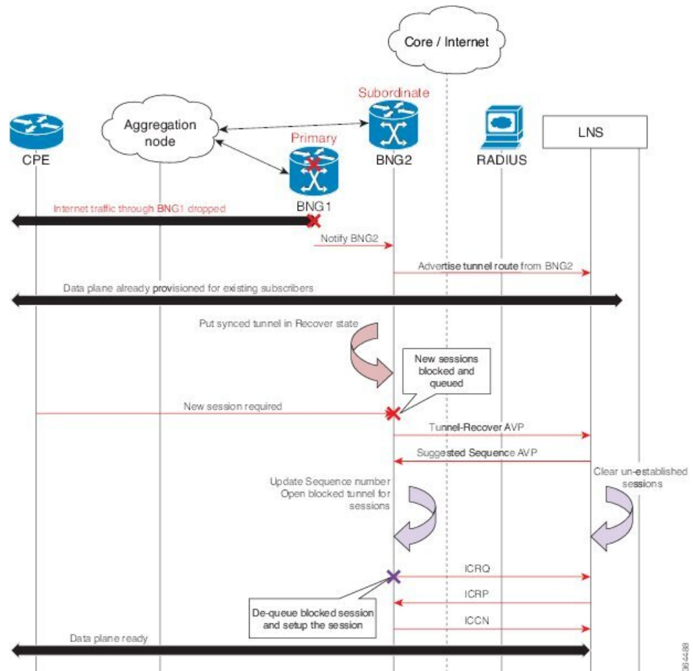
Figure 33: PPPoE-LAC Session Switchover
