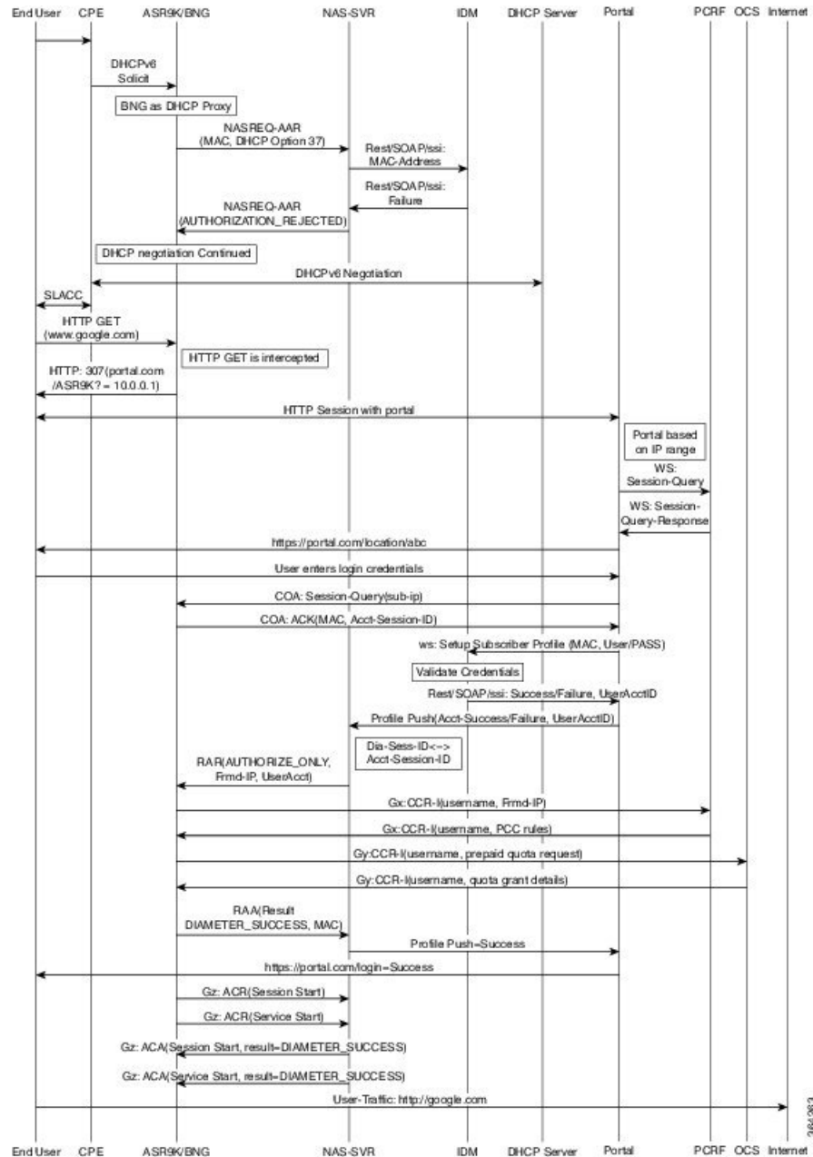
Figure 41: BNG DIAMETER Call Flow
