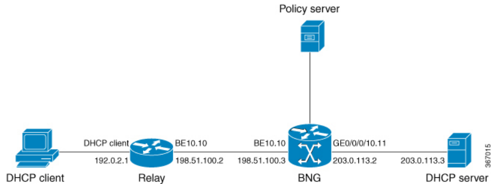
Figure 16: Network Topology of DHCP L3 Snooping in Cisco ASR 9000 BNG Router
