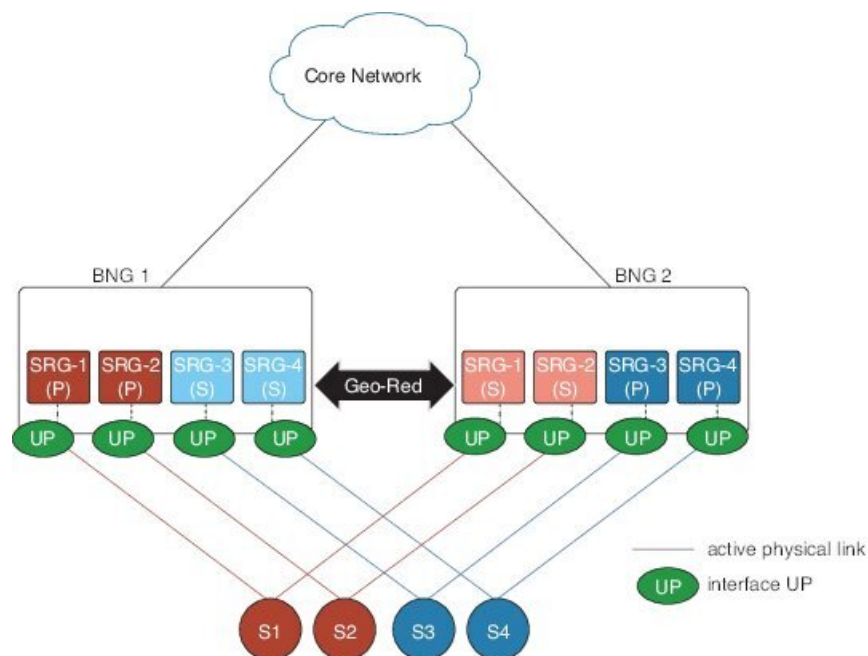
Figure 35: Active-active Session for BNG Geo Redundancy
