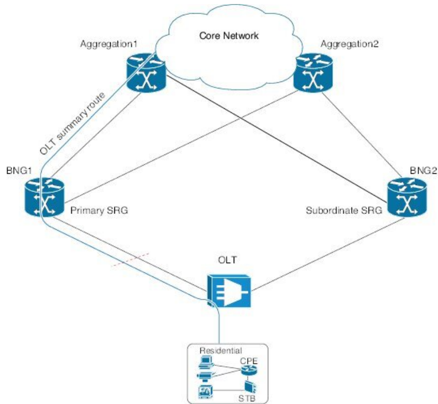
Figure 36: State Control Route for BNG Geo Redundancy
