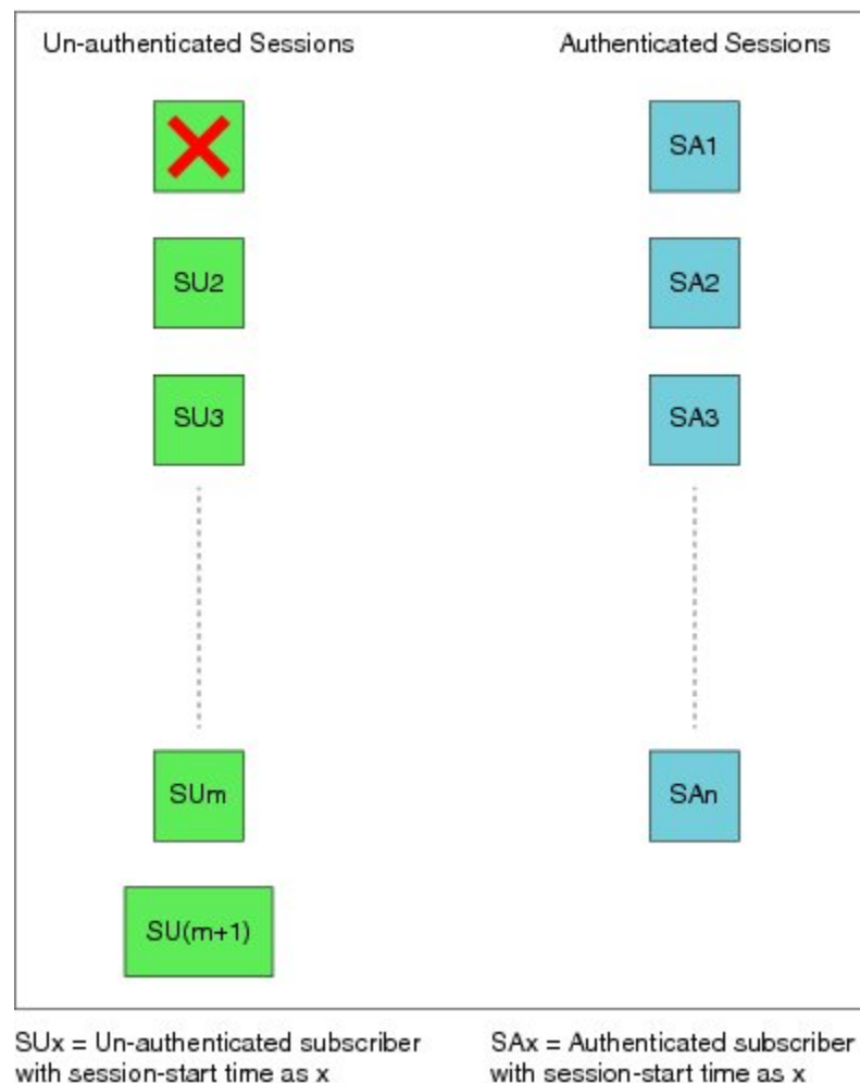
Figure 23: Subscriber Session Limit
