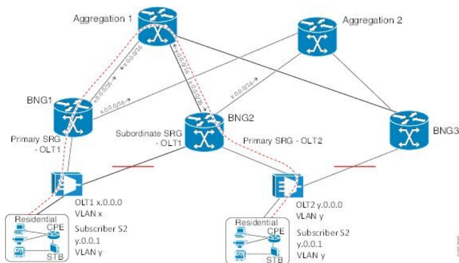
Figure 37: Peer-to-peer Traffic Flow with BNG Geo Redundancy
