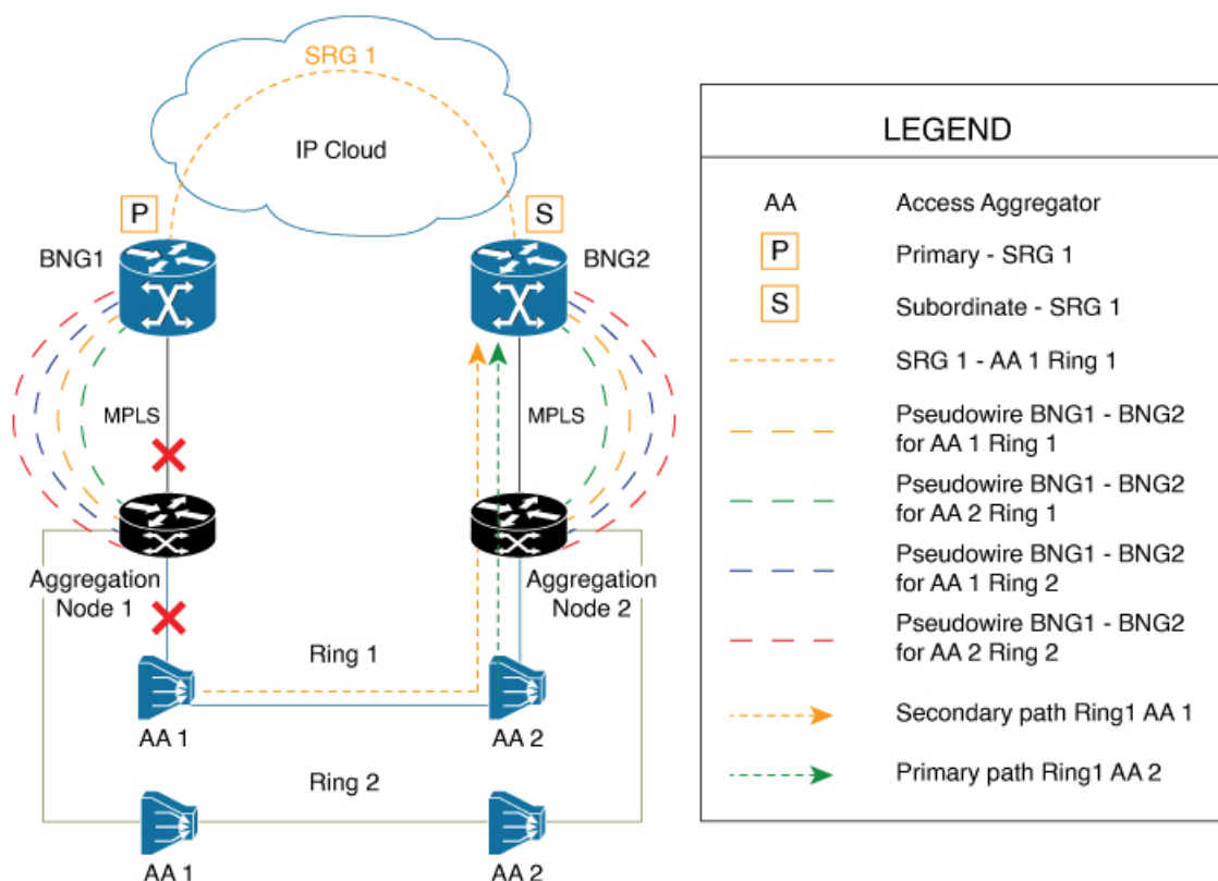
Figure 39: Link Failure Scenarios in BNG PWHE topology with SRG
