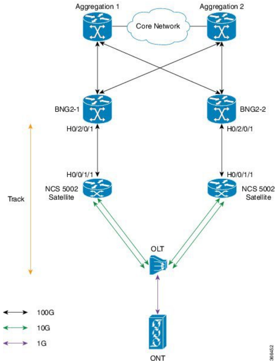
Figure 34: BNG Geo Redundancy with Cisco NCS 5000 Series nV Satellite
