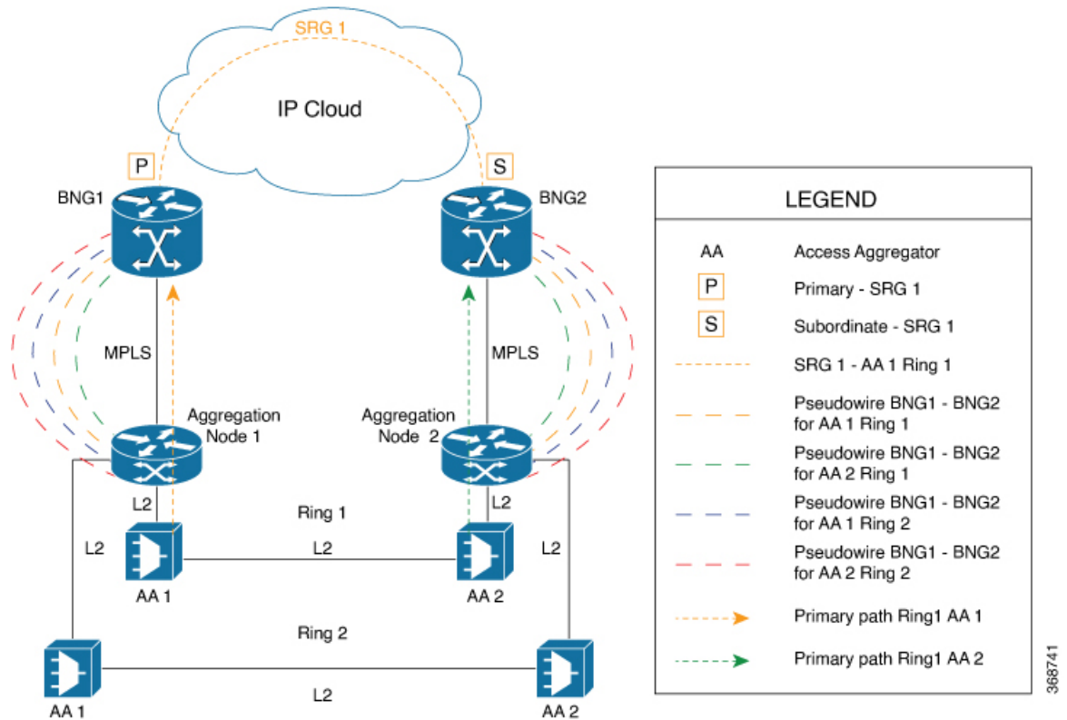
Figure 38: Sample Network Topology of SRG for PWHE Subscriber Sessions on BNG
