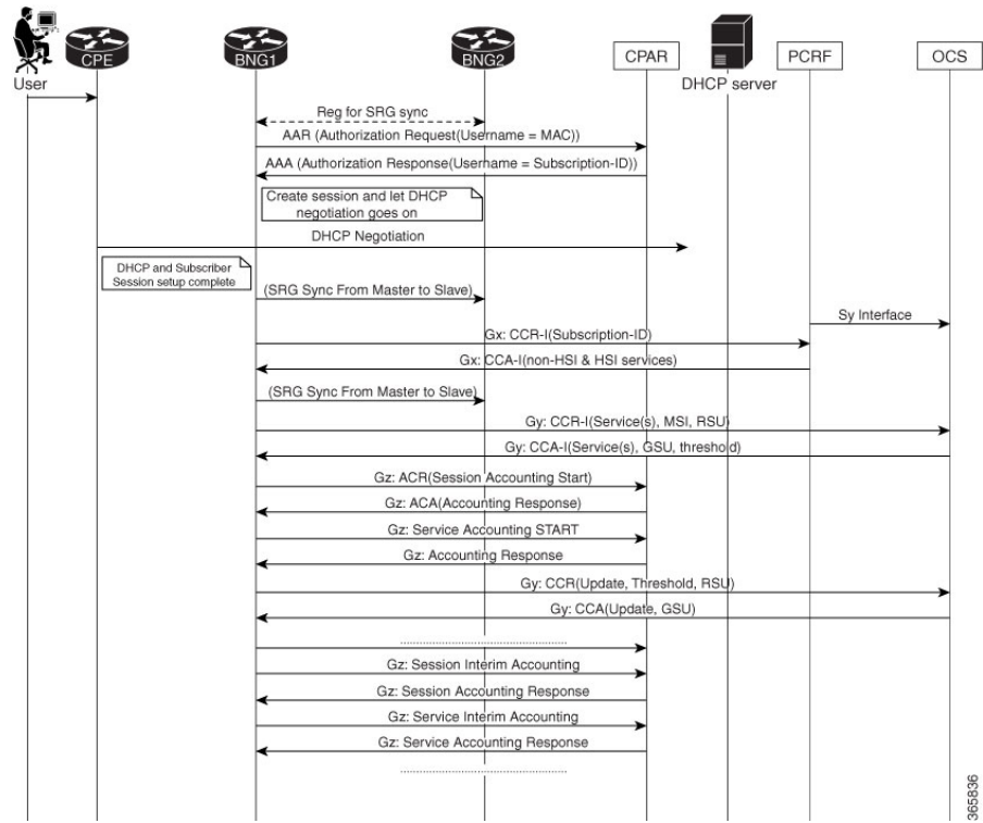
Figure 43: Call Flow of Subscriber Session Establishment With BNG DIAMETER-Geo Redundancy
