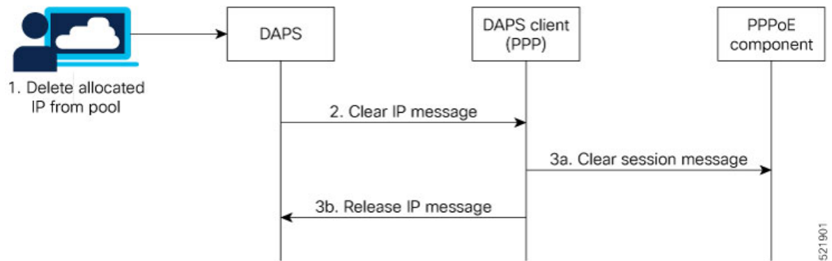
Figure 25: Call Flow of Dynamic Modification of DAPS Pool
