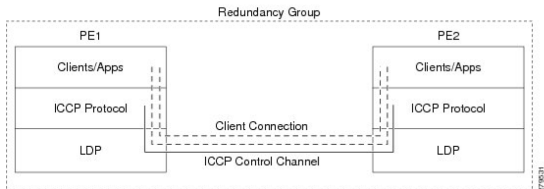
Figure 18: ICCP Protocol
