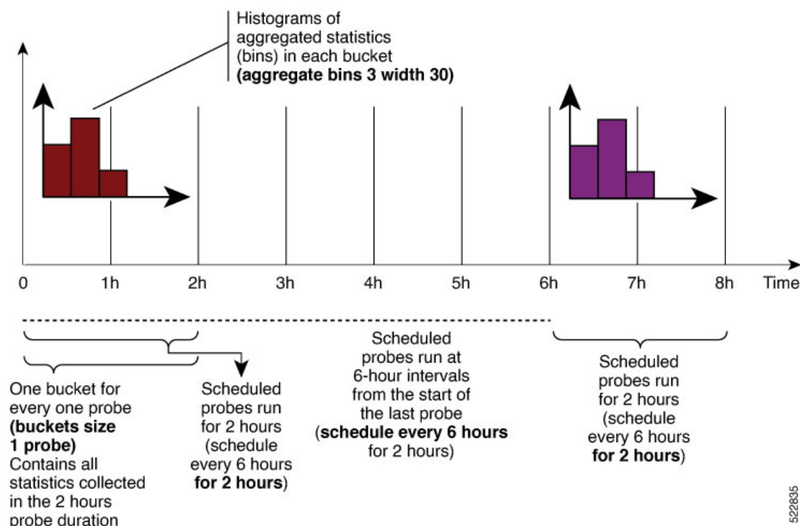
Figure 13: SLA Probe Scheduling Operation With Bin Aggregation
