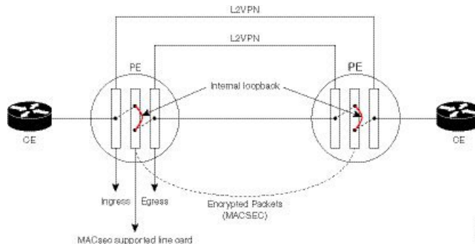
Figure 12: MACsec in an L2VPN topology
