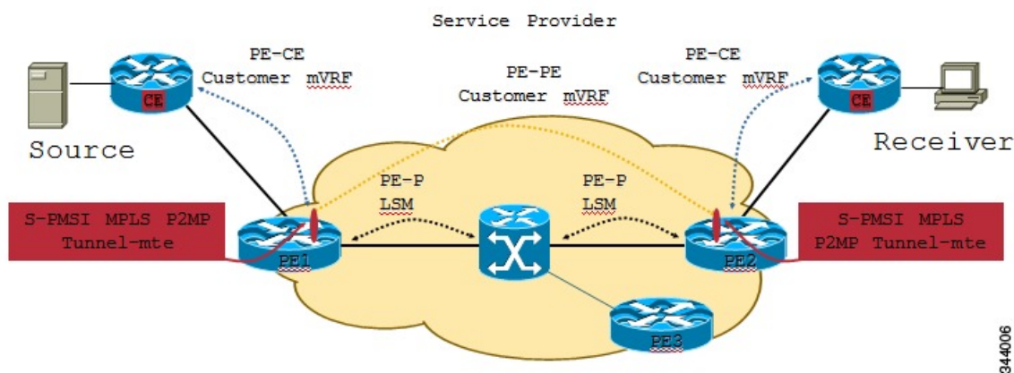
Figure 7: Multicast VRF
