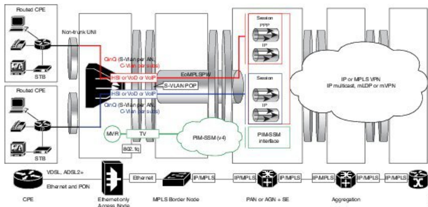
Figure 49: 1:1 deployment model for residential subscribers on PWHE
