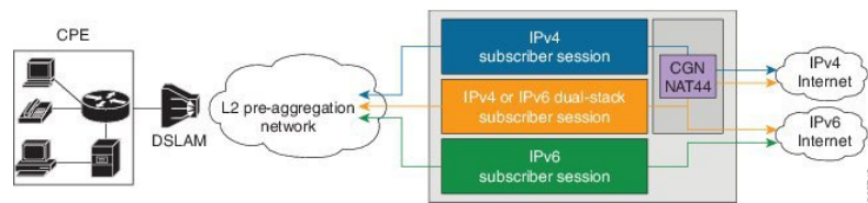
Figure 50: Deployment Model of Dual-Stack Subscriber Sessions
