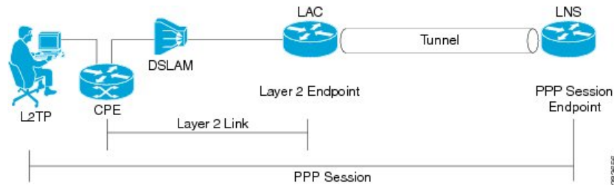
Figure 14: LAC Session
