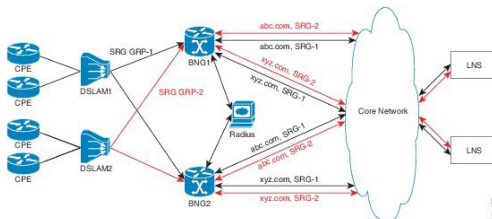
Figure 34: PPPoE-LAC Geo Redundancy Topology
