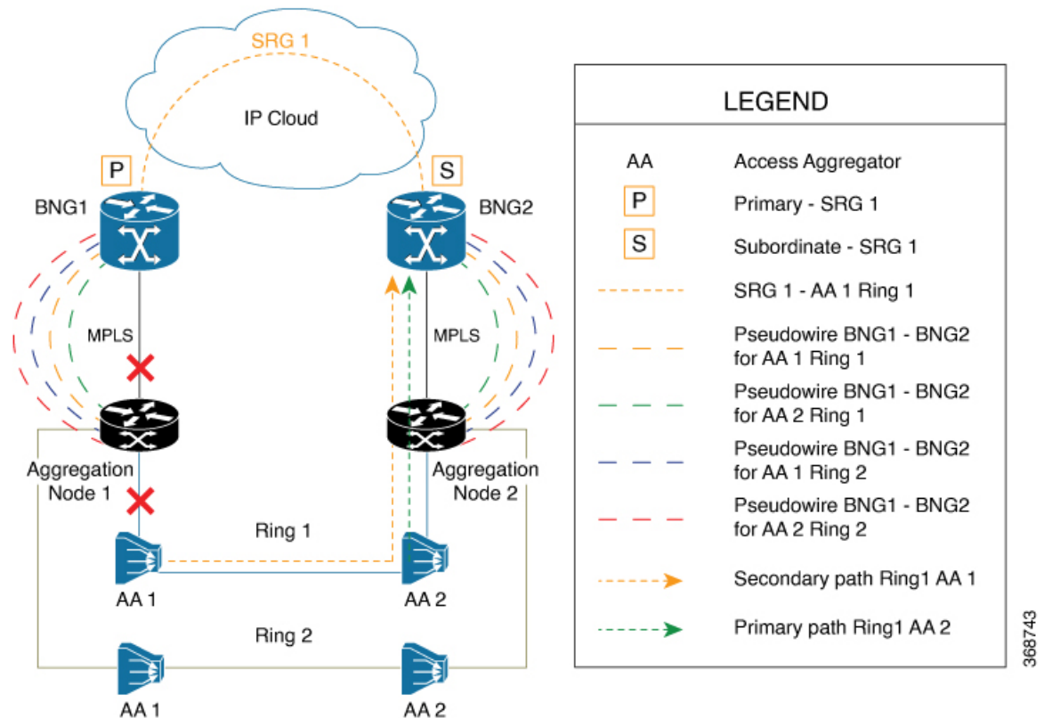
Figure 41: Link Failure Scenarios in BNG PWHE topology with SRG
