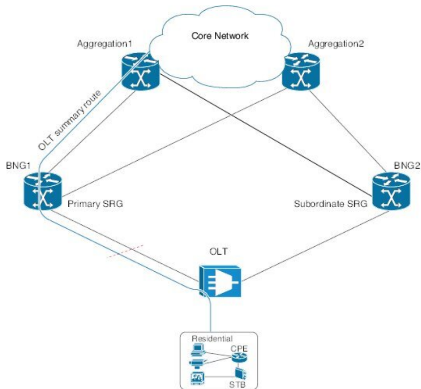
Figure 38: State Control Route for BNG Geo Redundancy
