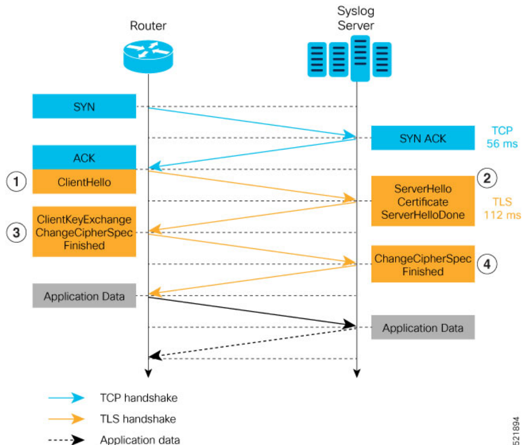
Figure 12: TLS Handshake
