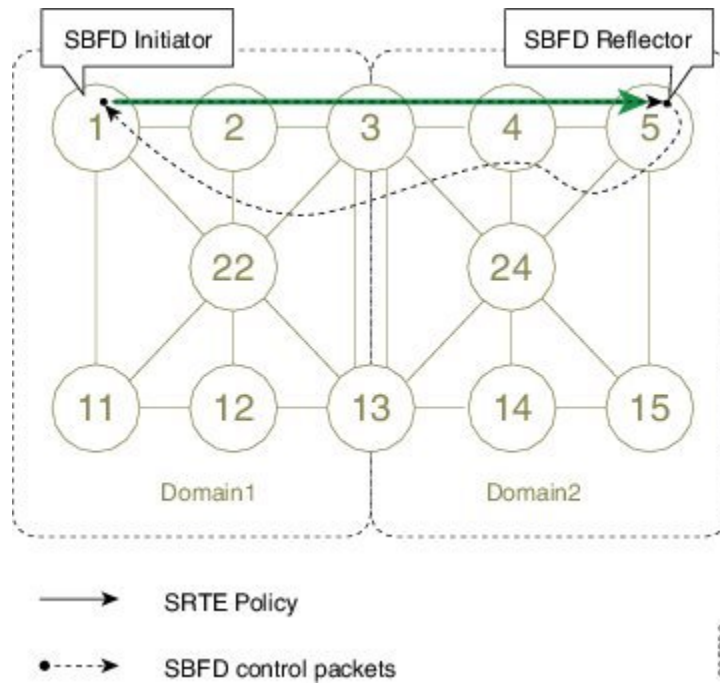
Figure 6: SBFDR Initiator and Reflector
