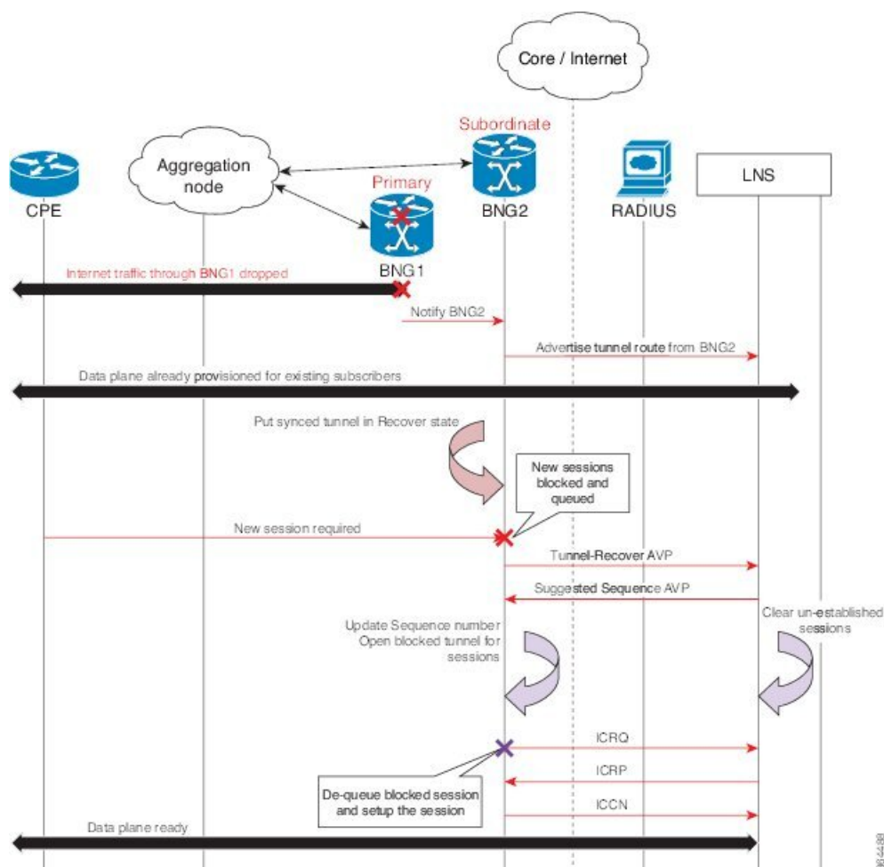
Figure 8: PPPoE-LAC Session Switchover
