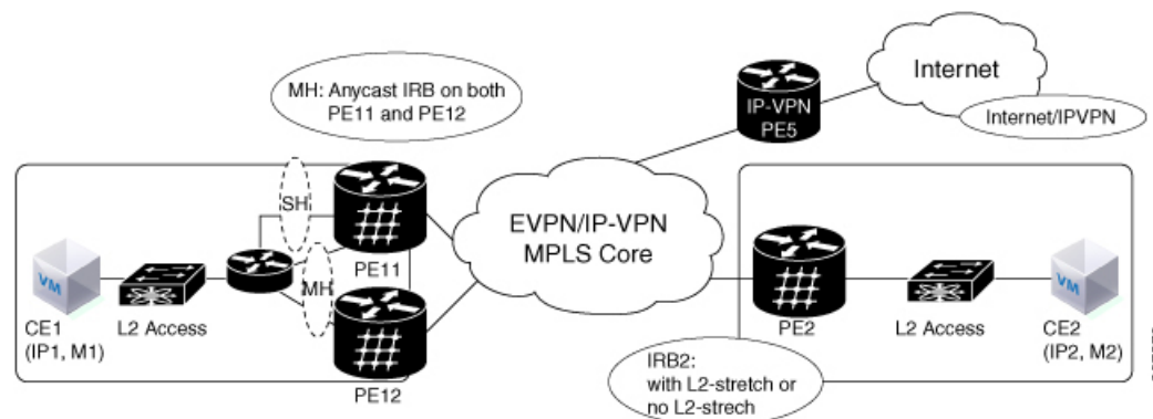
Figure 3: EVPN IRB with ASR 9000 as Centralized DCI Gateway
