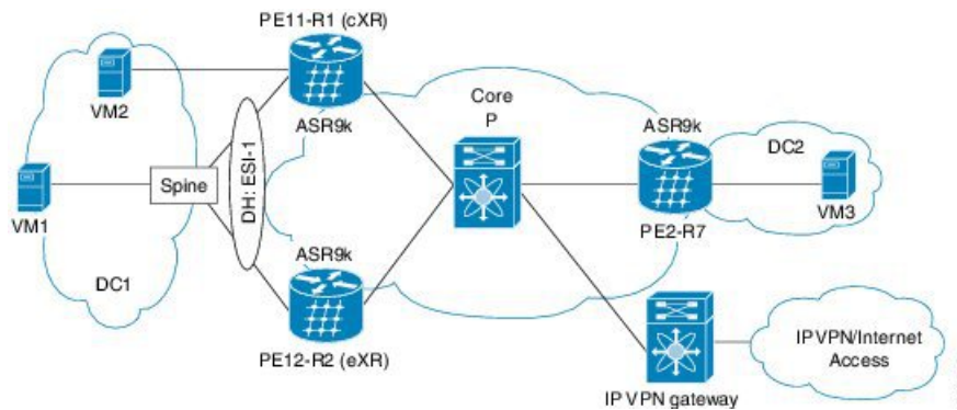
Figure 1: EVPN IRB
