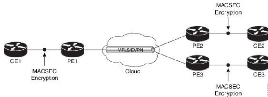
Figure 6: MACSec in a VPLS/EVPN Cloud
