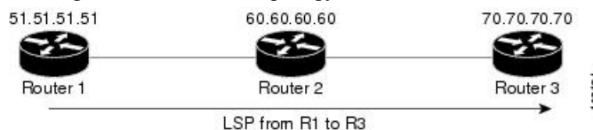
Figure 3: Sample Topology
