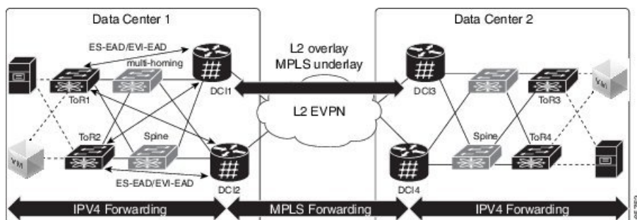
Figure 81: EVPN ESI Multipath
