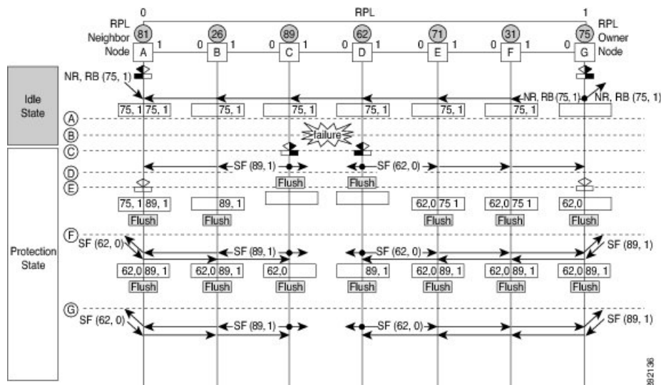
Figure 27: G.8032 Single Link Failure
