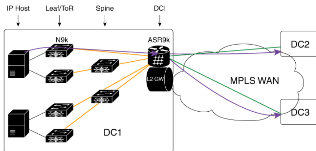
Figure 85: Single Homing VXLAN L2 GW
