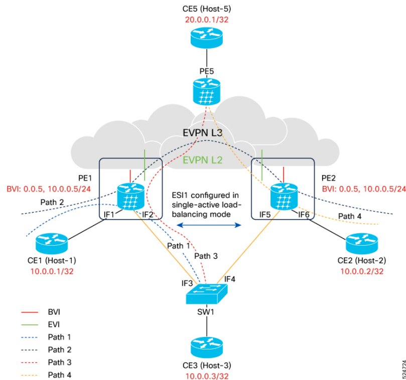
Figure 91: EVPN IRB multi-homing network topology
