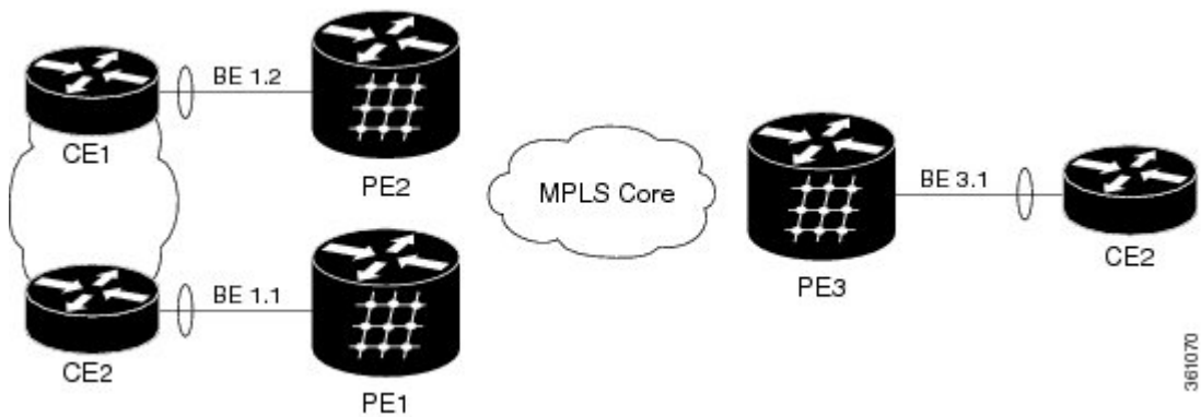
Figure 56: PBB-EVPN Multi Homed Network
