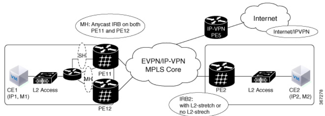
Figure 92: EVPN IRB with ASR 9000 as Centralized DCI Gateway
