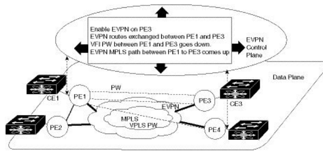
Figure 82: EVPN MPLS Seamless Integration with VPLS
