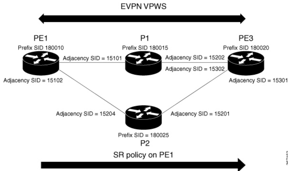
Figure 93: EVPN VPWS Preferred Path over SR-TE Policy
