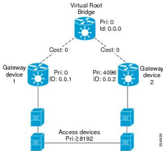
Figure 64: MSTAG Guidelines
