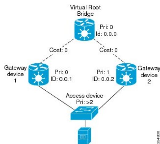
Figure 68: PVSTAG Guidelines
