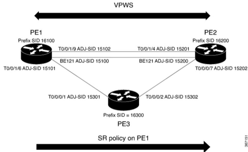
Figure 94: L2VPN VPWS and VPLS Preferred Path over SR-TE Policy
