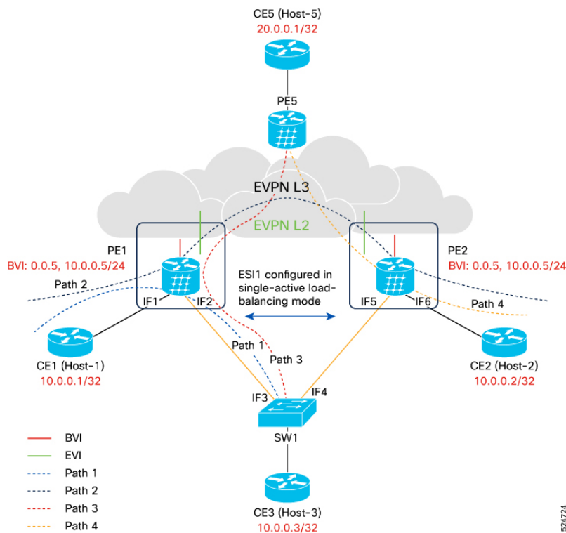
Figure 90: EVPN IRB single-homing network topology
