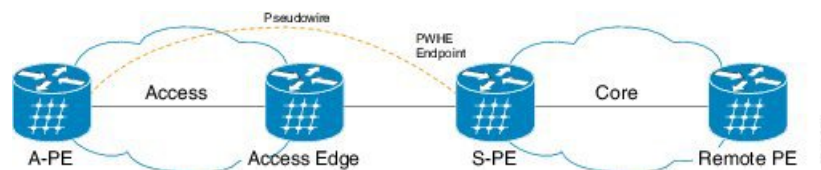
Figure 30: Pseudowire Network
