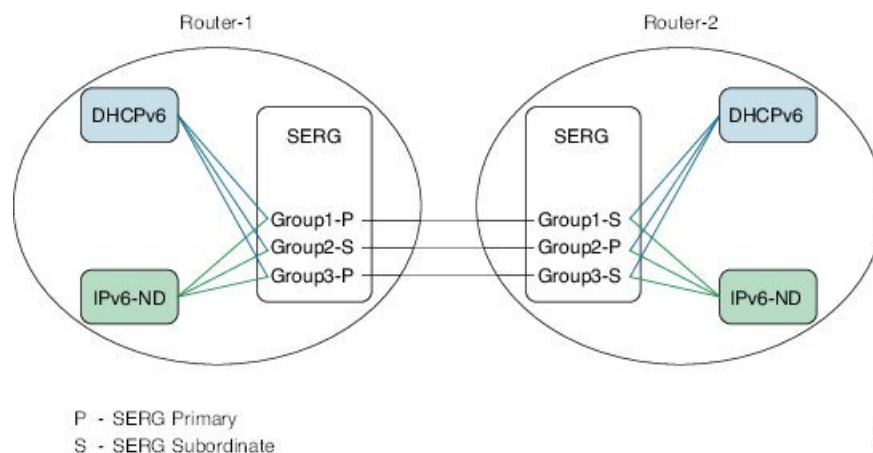
Figure 13: Geo Redundancy with Multiple SERGs
