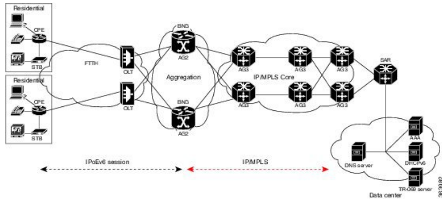
Figure 59: Sample Deployment Topology for Routed Subscriber Sessions
