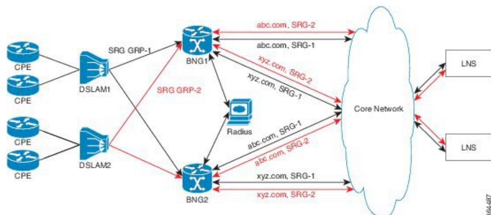
Figure 31: PPPoE-LAC Geo Redundancy Topology
