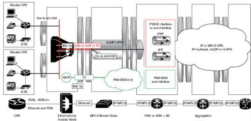
Figure 45: N:1 deployment model for residential subscribers on PWHE
