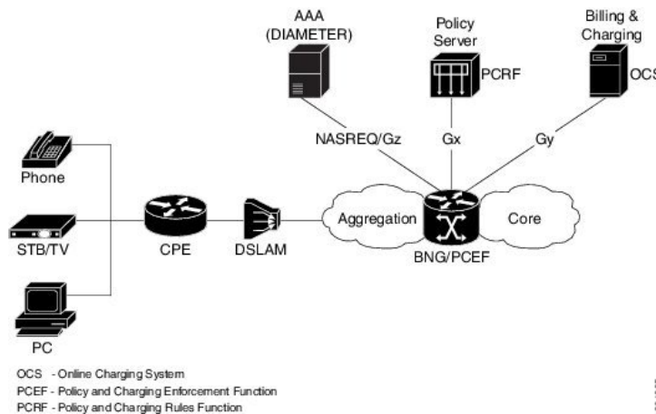
Figure 39: DIAMETER Interface in BNG
