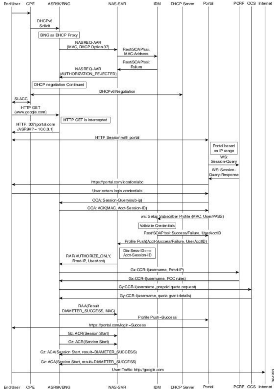
Figure 40: BNG DIAMETER Call Flow
