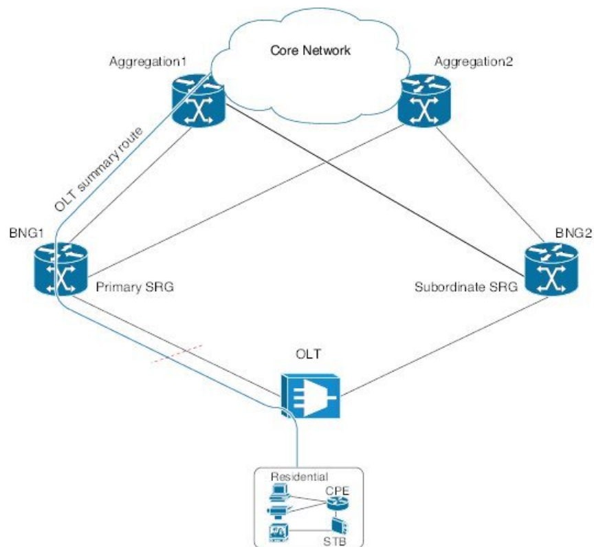
Figure 35: State Control Route for BNG Geo Redundancy
