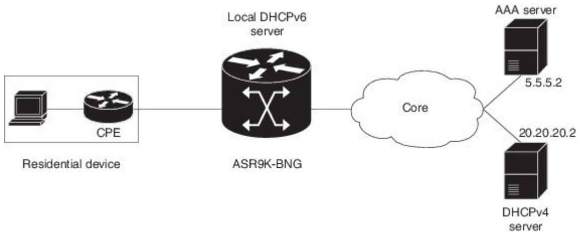
Figure 57: Sample topology for Dual-Stack
