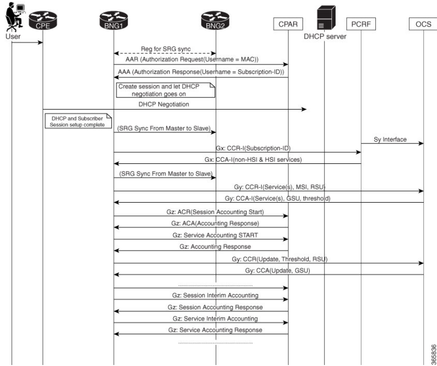
Figure 42: Call Flow of Subscriber Session Establishment With BNG DIAMETER-Geo Redundancy
