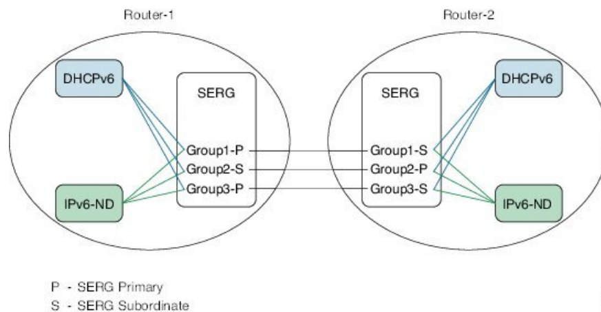
Figure 30: Geo Redundancy with Multiple SERGs
