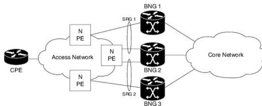
Figure 26: BNG Subscriber Redundancy Group
