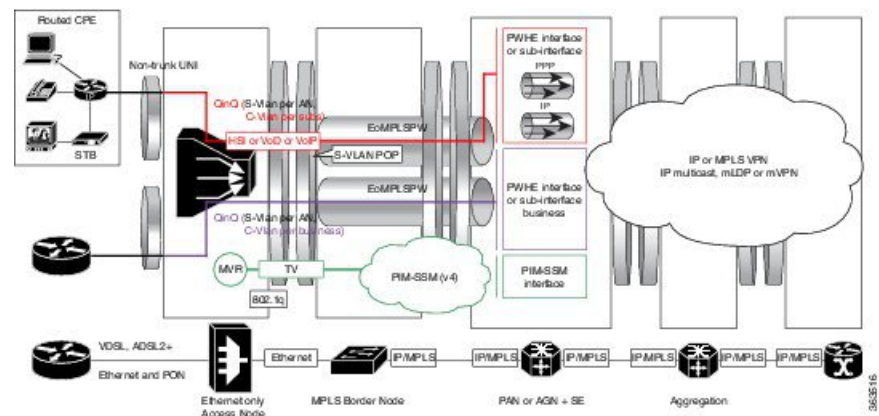
Figure 48: Deployment Model 2 for Residential and Business Subscribers on PWHE
