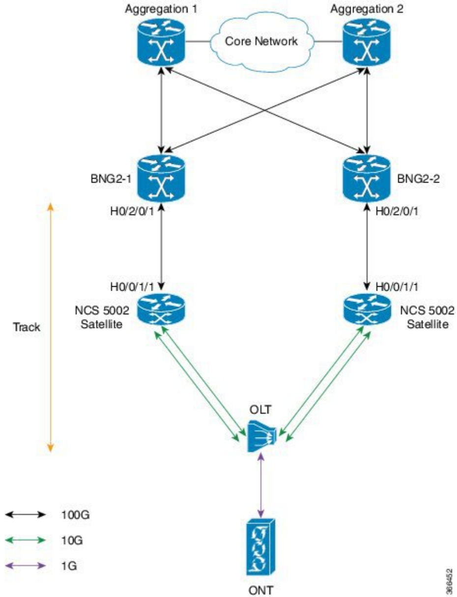
Figure 33: BNG Geo Redundancy with Cisco NCS 5000 Series nV Satellite
