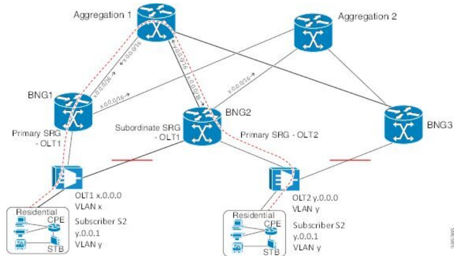
Figure 36: Peer-to-peer Traffic Flow with BNG Geo Redundancy
