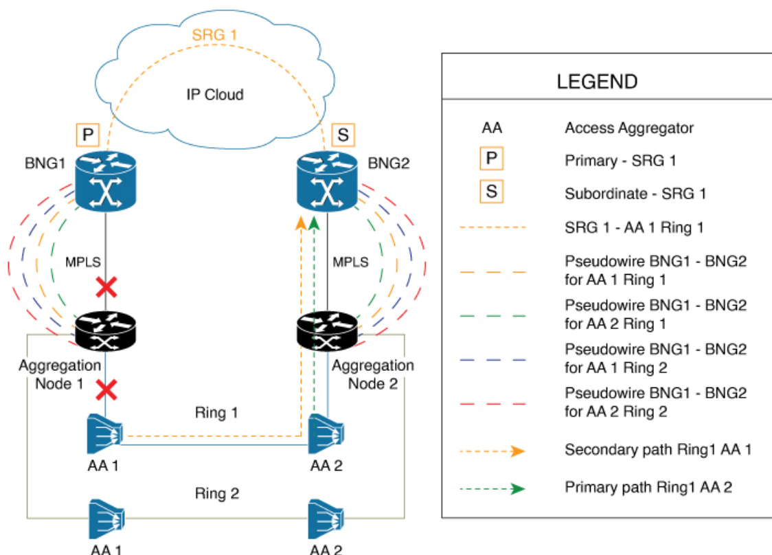
Figure 38: Link Failure Scenarios in BNG PWHE topology with SRG
