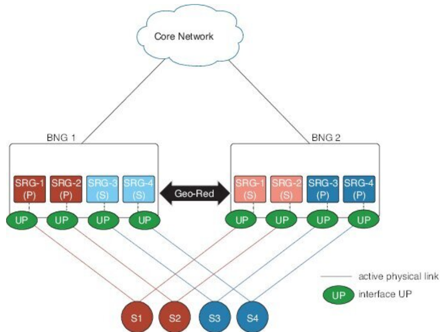
Figure 34: Active-active Session for BNG Geo Redundancy
