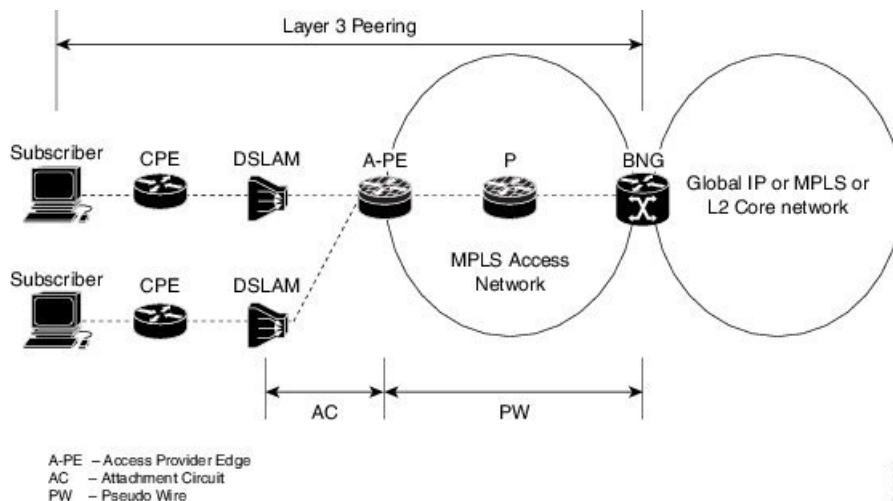
Figure 44: Sample Topology for BNG over Pseudowire Headend
