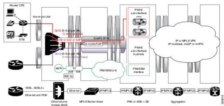
Figure 47: Deployment Model 1 for Residential and Business Subscribers on PWHE
