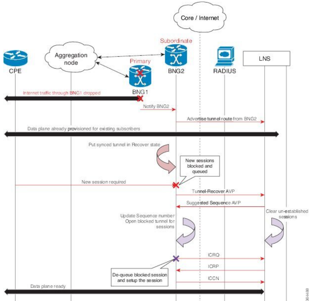
Figure 32: PPPoE-LAC Session Switchover
