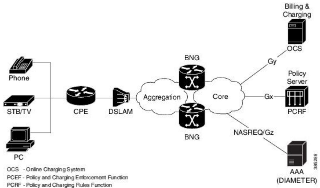
Figure 41: DIAMETER-Geo Redundancy Interworking
