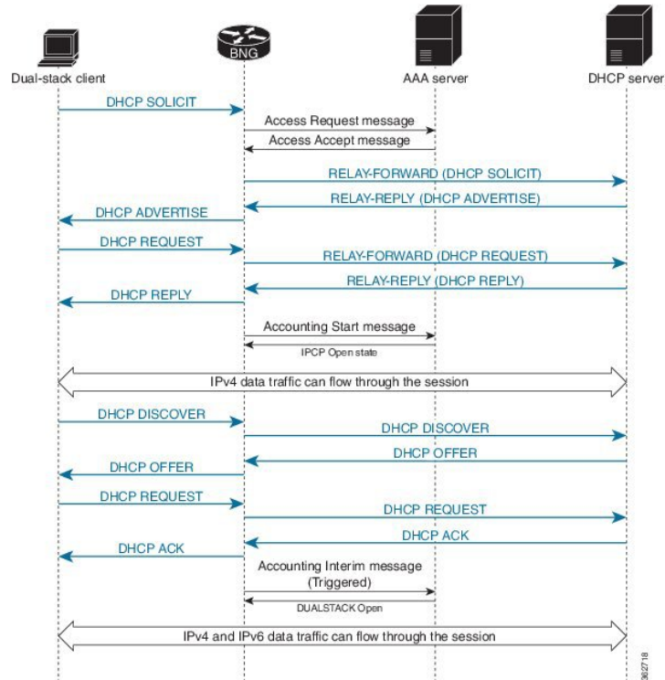
Figure 56: Call Flow of IPoE Dual-Stack - IPv6 Address-Family Starts First
