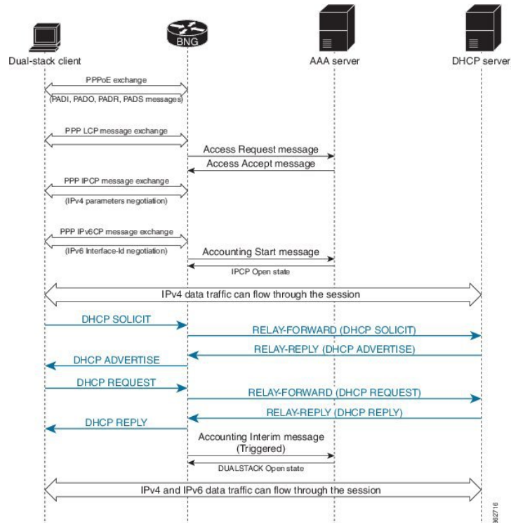
Figure 54: Call Flow of PPPoE Dual-Stack - DHCPv6-Based Address Assignment
