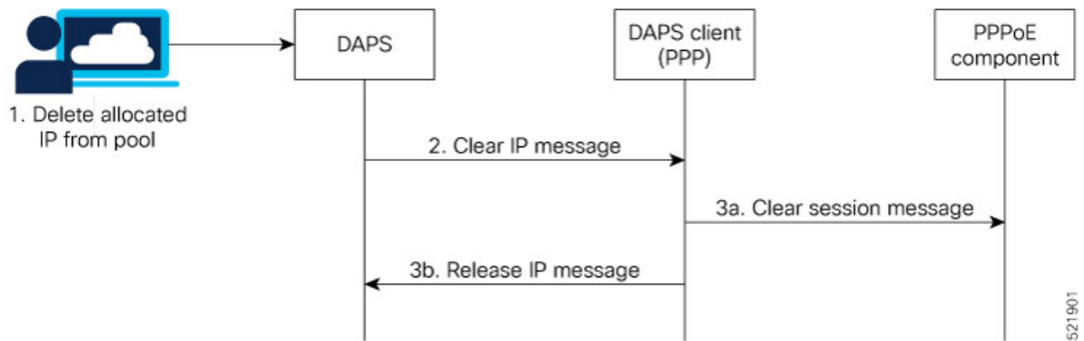
Figure 23: Call Flow of Dynamic Modification of DAPS Pool
