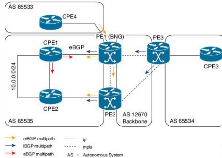
Figure 58: Sample topology for eBGP over PPPoE
