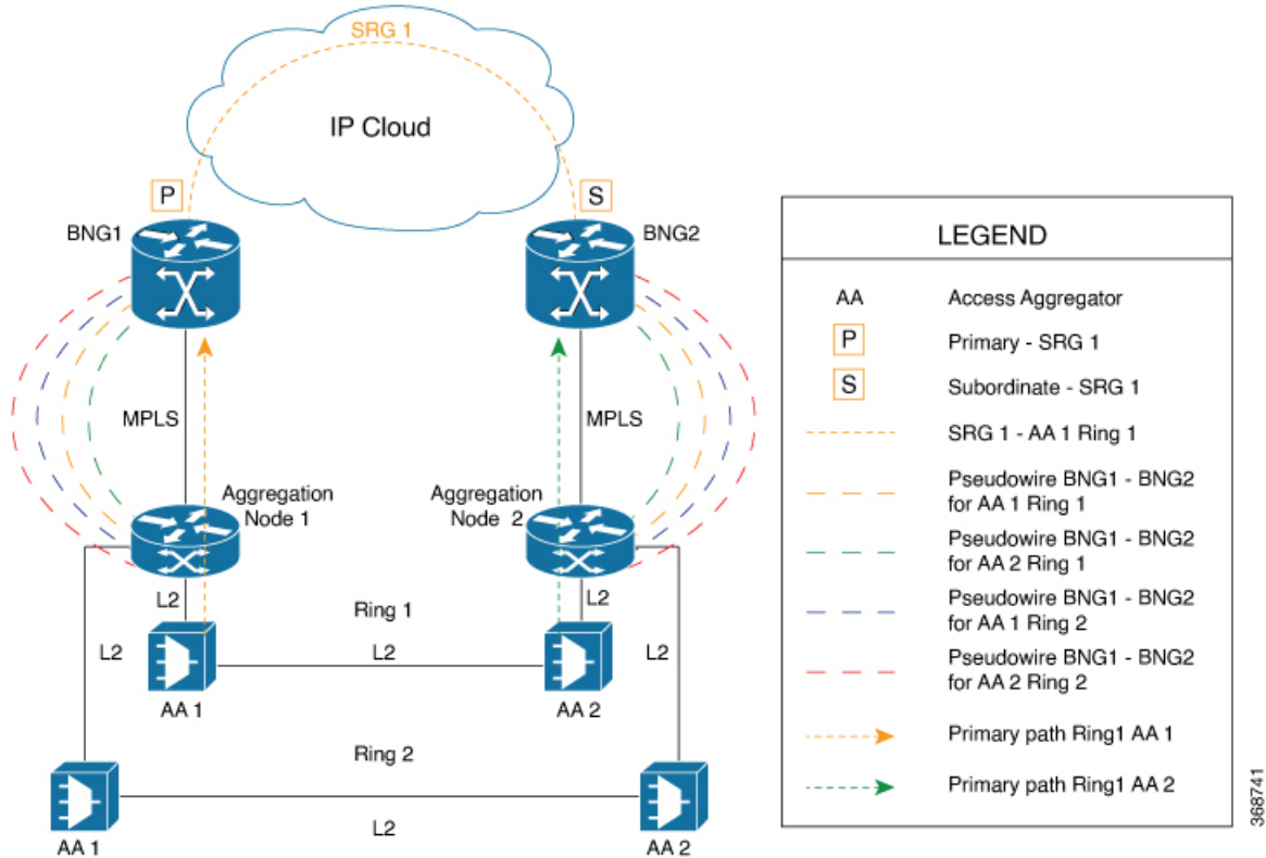
Figure 37: Sample Network Topology of SRG for PWHE Subscriber Sessions on BNG
