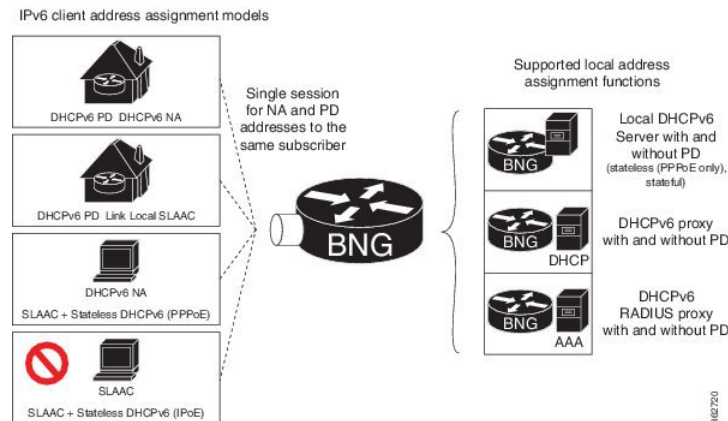
Figure 50: IPv6 Client Address Assignment Models
