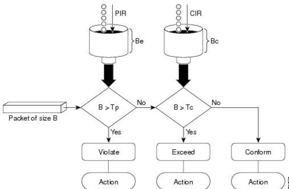
Figure 5: Marking Packets and Assigning Actions—2-Rate Policer
