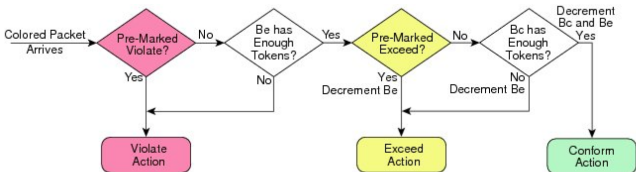
Figure 4: 2R3C Policing Process Flowchart
