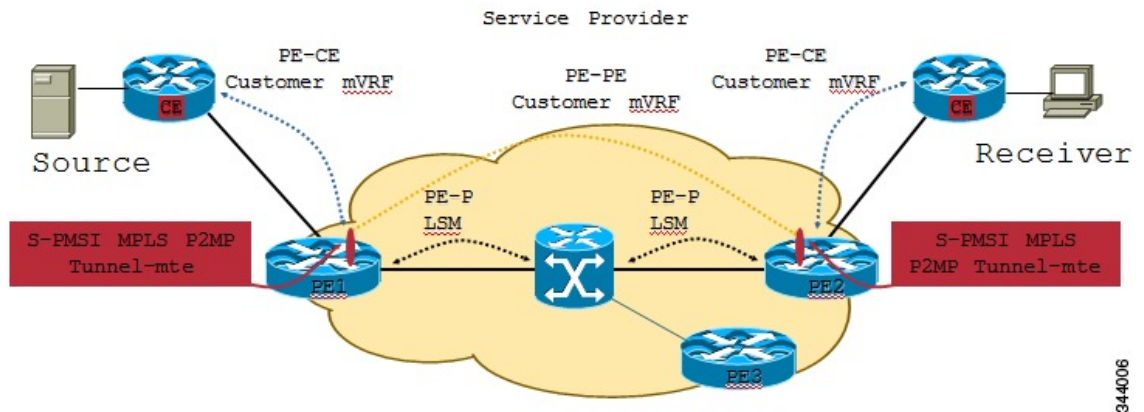
Figure 6: Multicast VRF
