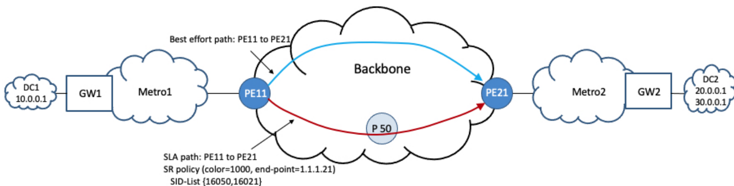
Figure 14: Backbone Transport Paths (Traffic Direction – DC1 to DC2)
