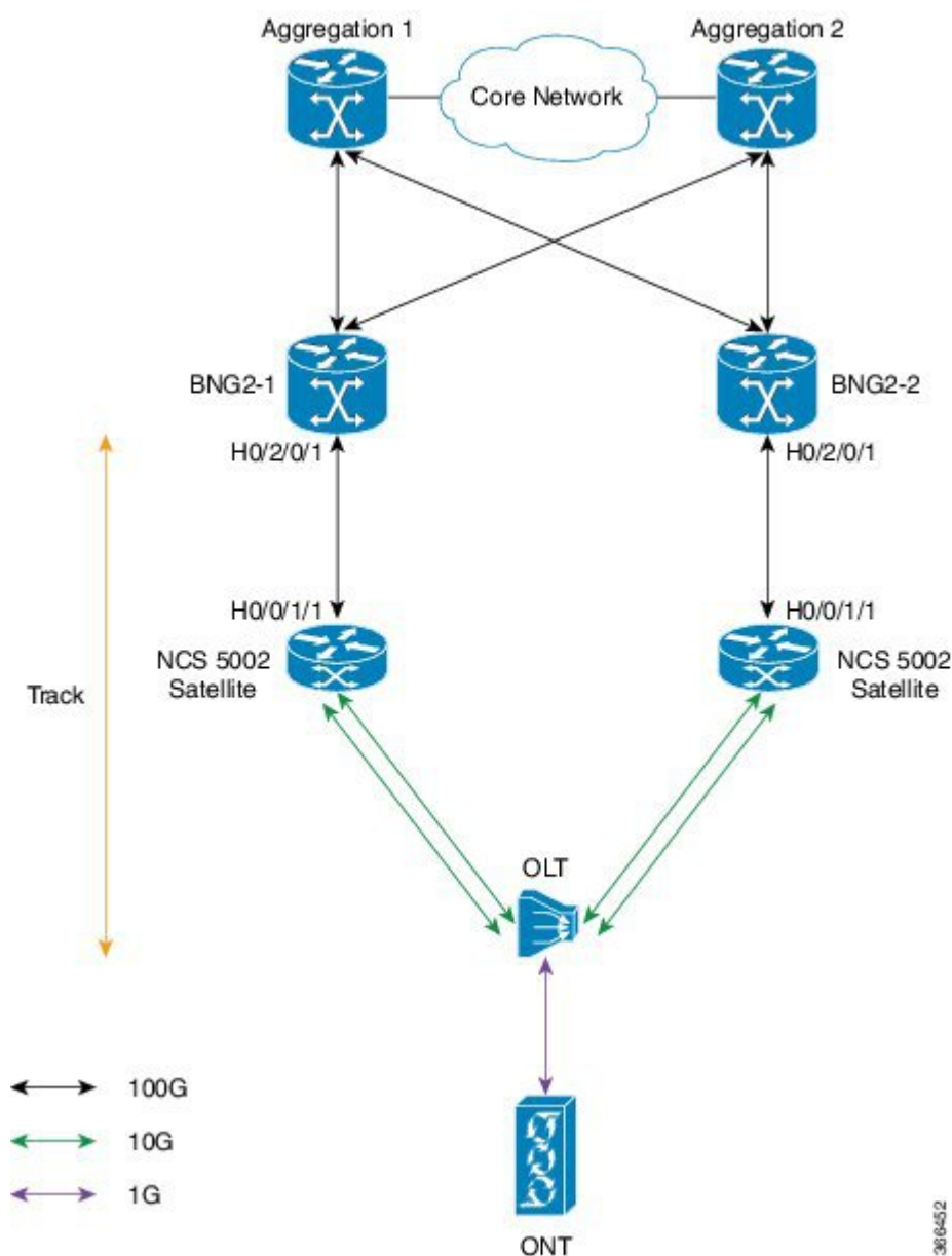
Figure 7: BNG Geo Redundancy with Cisco NCS 5000 Series nV Satellite
