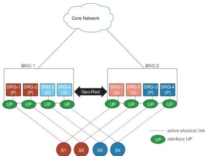
Figure 9: Active-active Session for BNG Geo Redundancy
