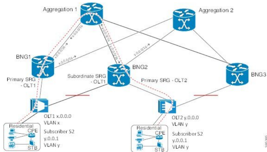
Figure 11: Peer-to-peer Traffic Flow with BNG Geo Redundancy
