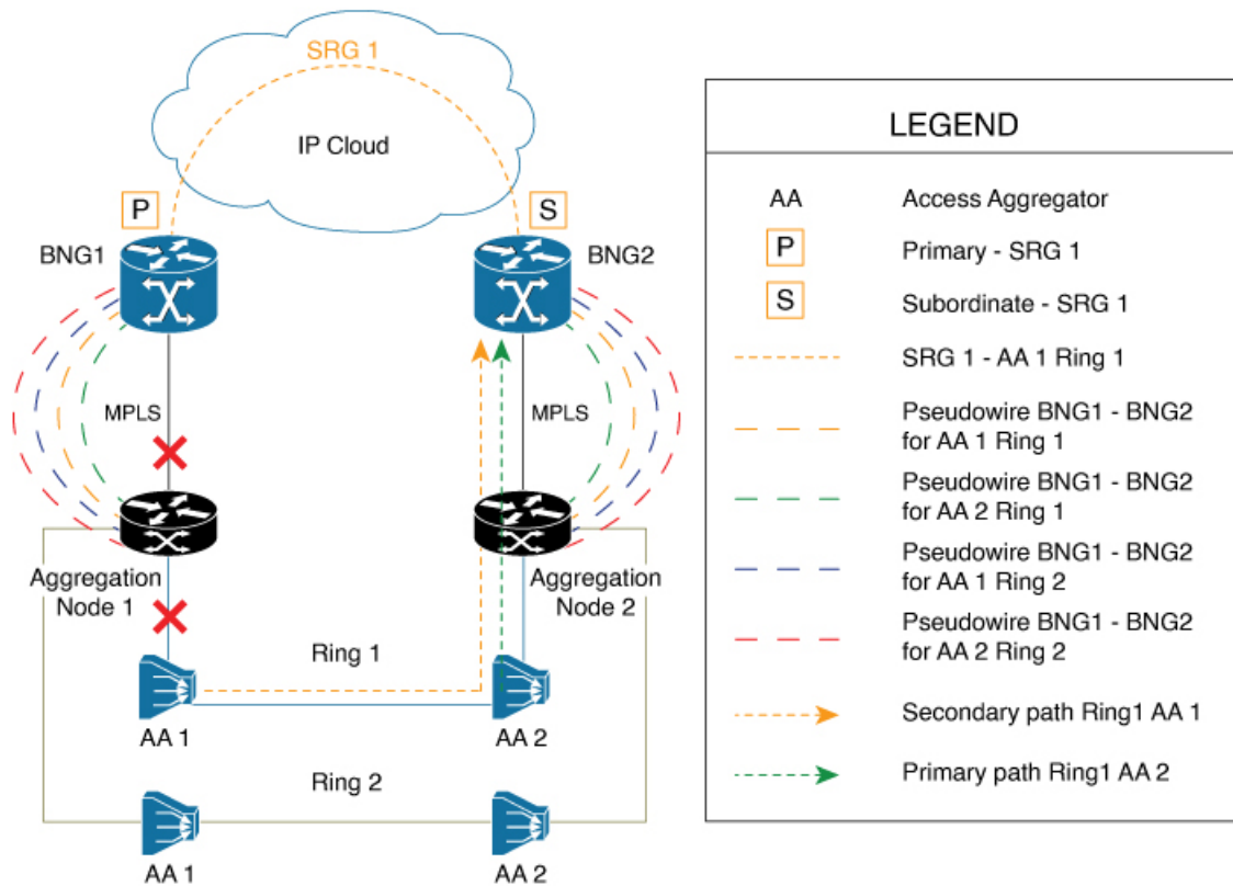
Figure 13: Link Failure Scenarios in BNG PWHE topology with SRG
