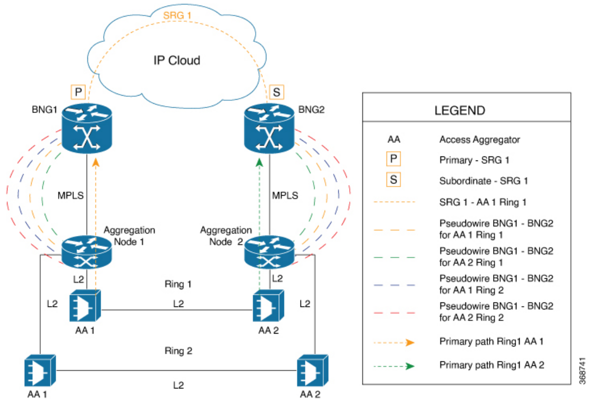
Figure 12: Sample Network Topology of SRG for PWHE Subscriber Sessions on BNG
