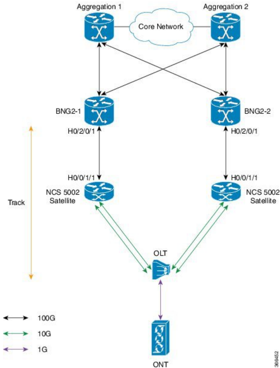
Figure 26: BNG Geo Redundancy with Cisco NCS 5000 Series nV Satellite
