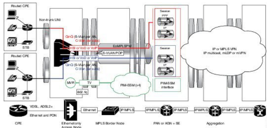
Figure 40: 1:1 deployment model for residential subscribers on PWHE
