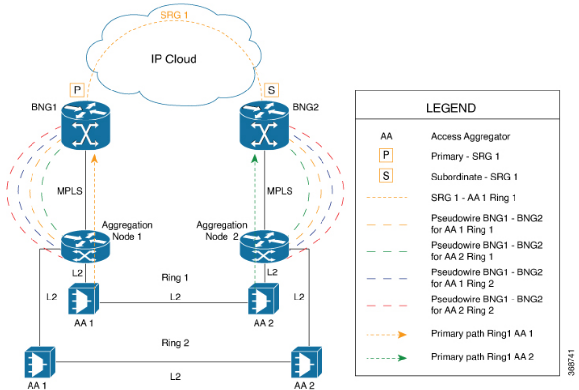
Figure 31: Sample Network Topology of SRG for PWHE Subscriber Sessions on BNG
