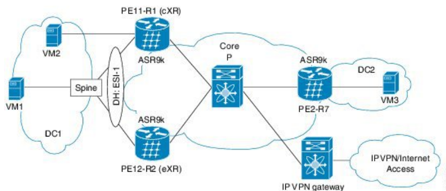
Figure 1: EVPN IRB
