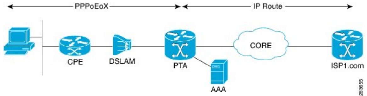
Figure 2: PPPoE-PTA Session
