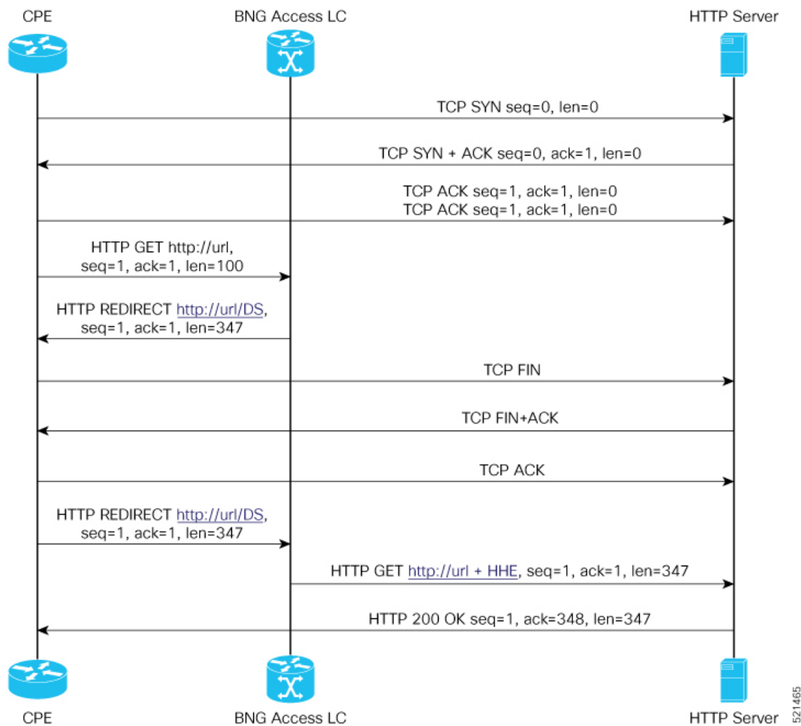
Figure 19: Sequence of events for HTTP Header Enrichment
