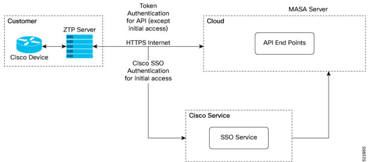
Figure 27: Components of the Authentication Flow
