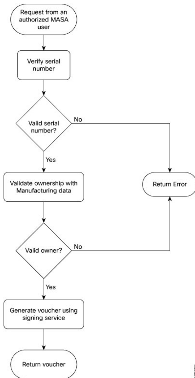
Figure 28: Workflow to Obtain Ownership Vouchers
