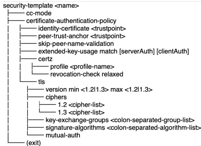
Figure 24: CLI Structure
