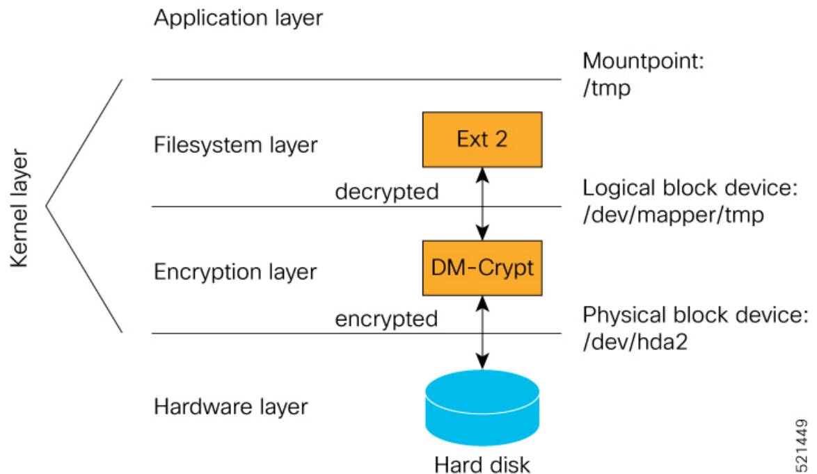
Figure 25: DM-Crypt Encryption
