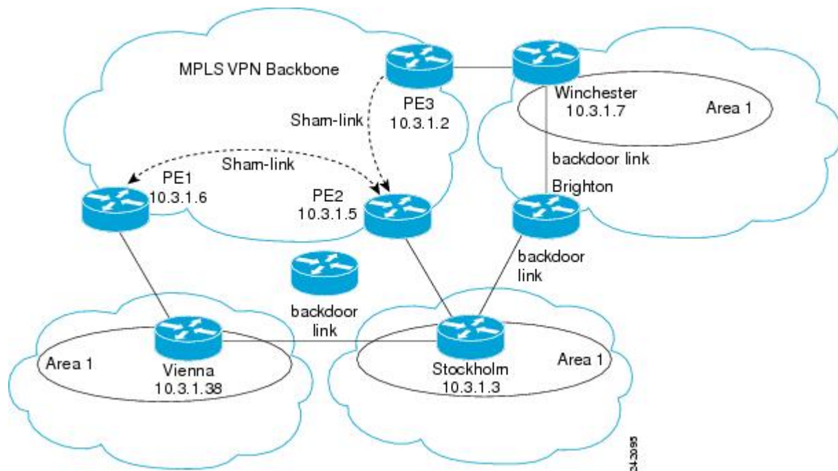
Figure 32: Sham Link Between PE Routers to Connected OSPF Client Sites
