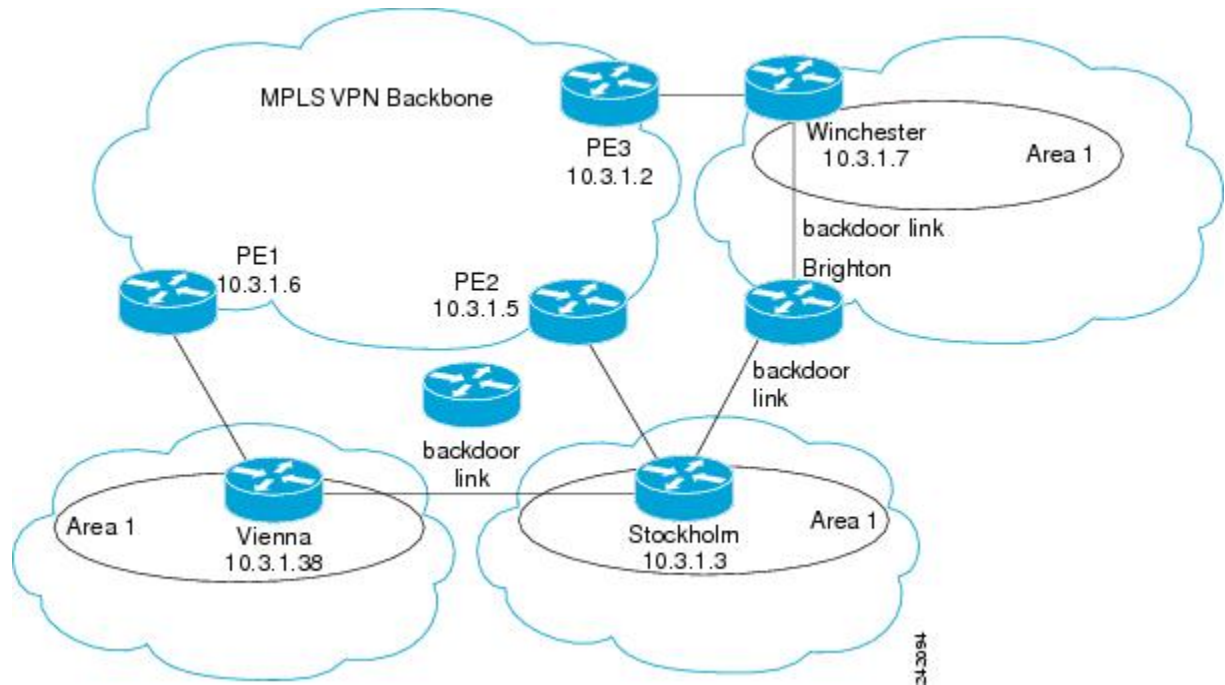
Figure 31: Backdoor Paths Between OSPF Client Sites
