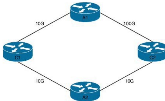
Figure 35: Unequal Cost Multipath for Static Routing
