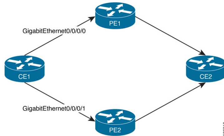
Figure 27: Traffic flow under metric fallback anomaly loss
