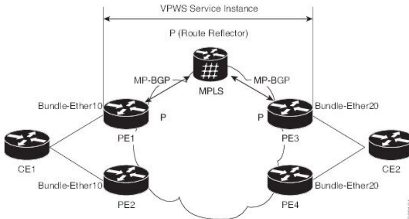
Figure 114: EVPN VPWS Multi-Homed
