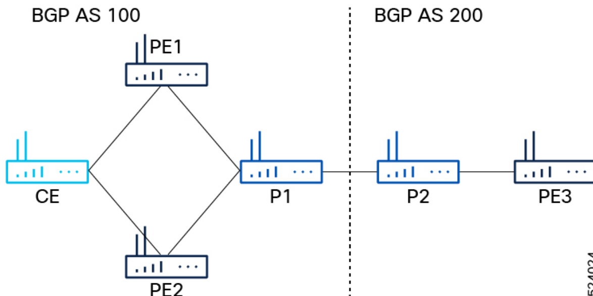
Figure 99: Inter-AS option C
