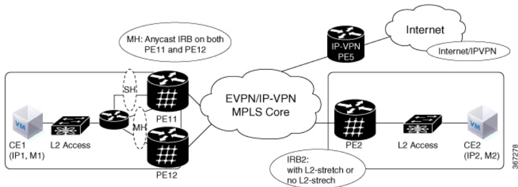
Figure 113: EVPN IRB with ASR 9000 as Centralized DCI Gateway
