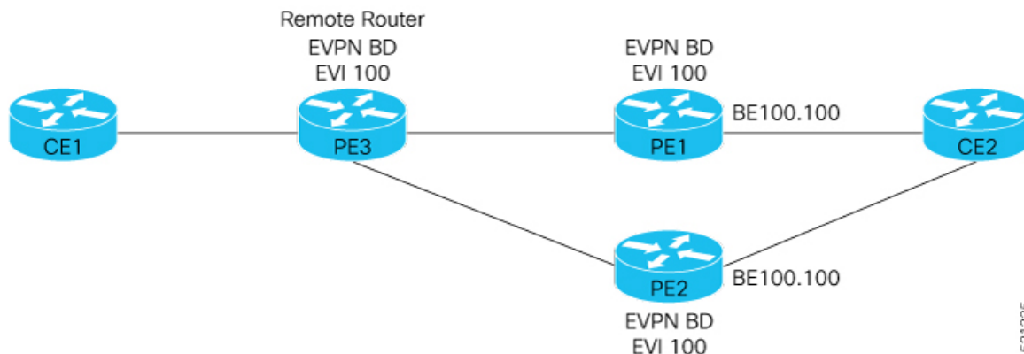
Figure 96: Layer 2 FRR multi-homing topology
