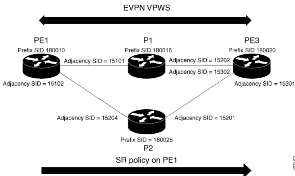
Figure 116: EVPN VPWS Preferred Path over SR-TE Policy
