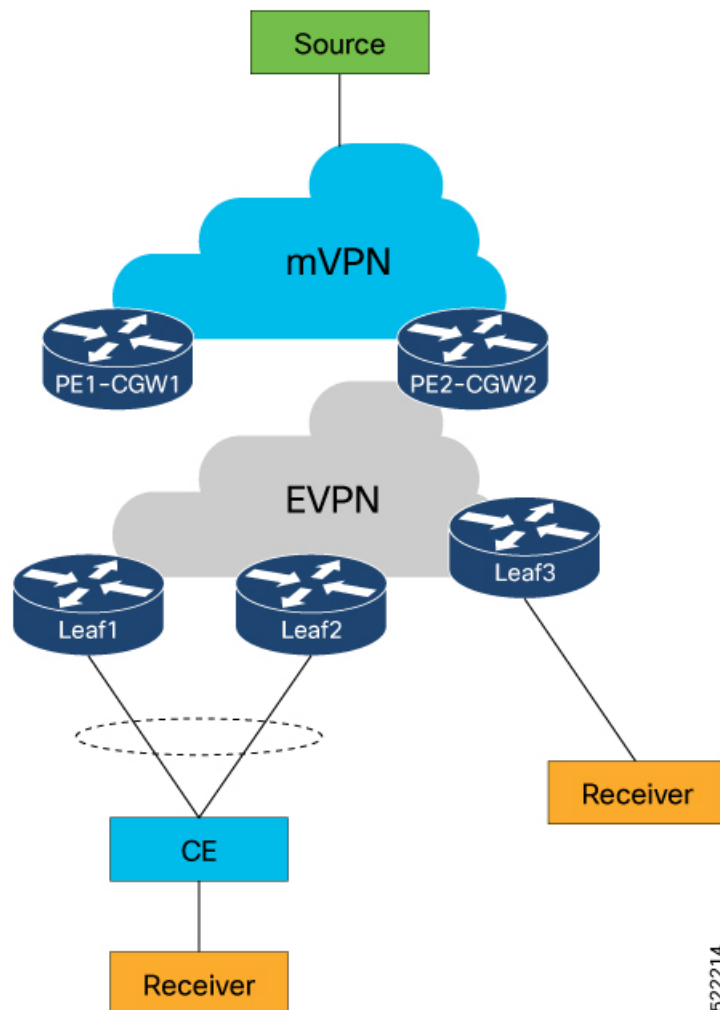
Figure 100: Topology
