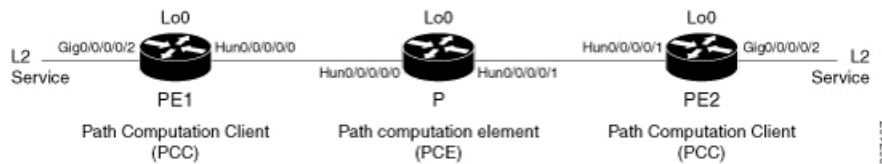
Figure 118: EVPN VPWS On Demand Next Hop with SR-TE
