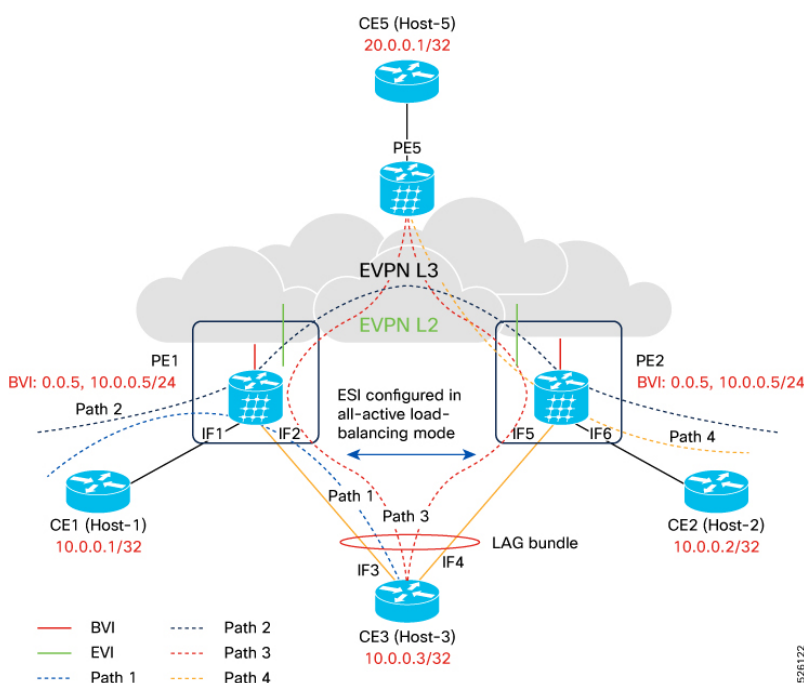
Figure 110: EVPN IRB multi-homing network topology
