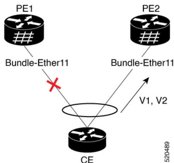
Figure 108: EVPN port-active manual switchover
