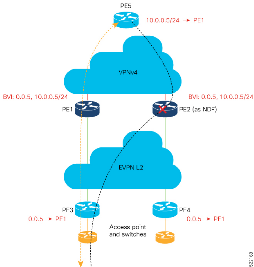
Figure 112: Topology
