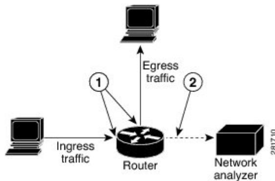
Figure 32: Network Analysis on a Cisco ASR 9000 Router With Traffic Mirroring
