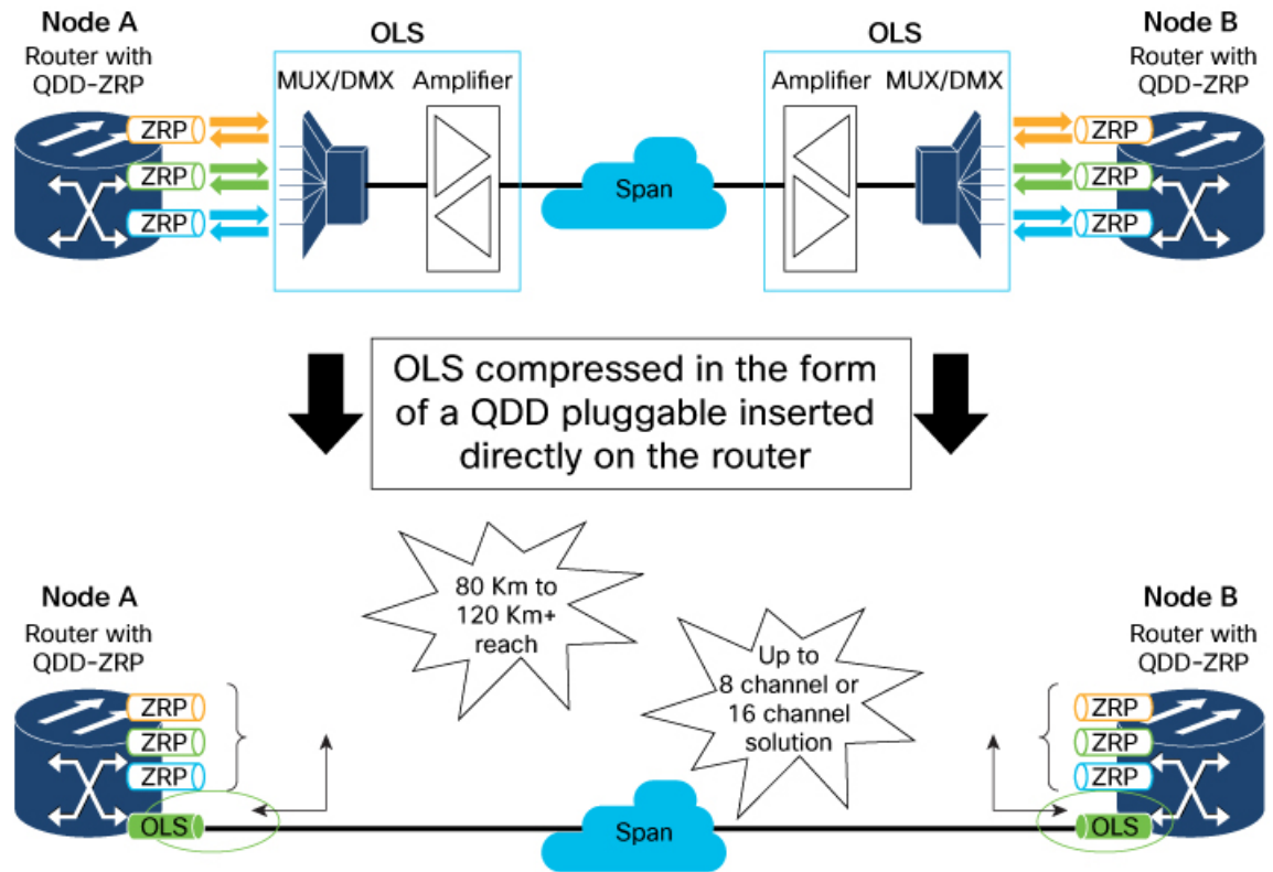
Figure 35: QDD optical line system
