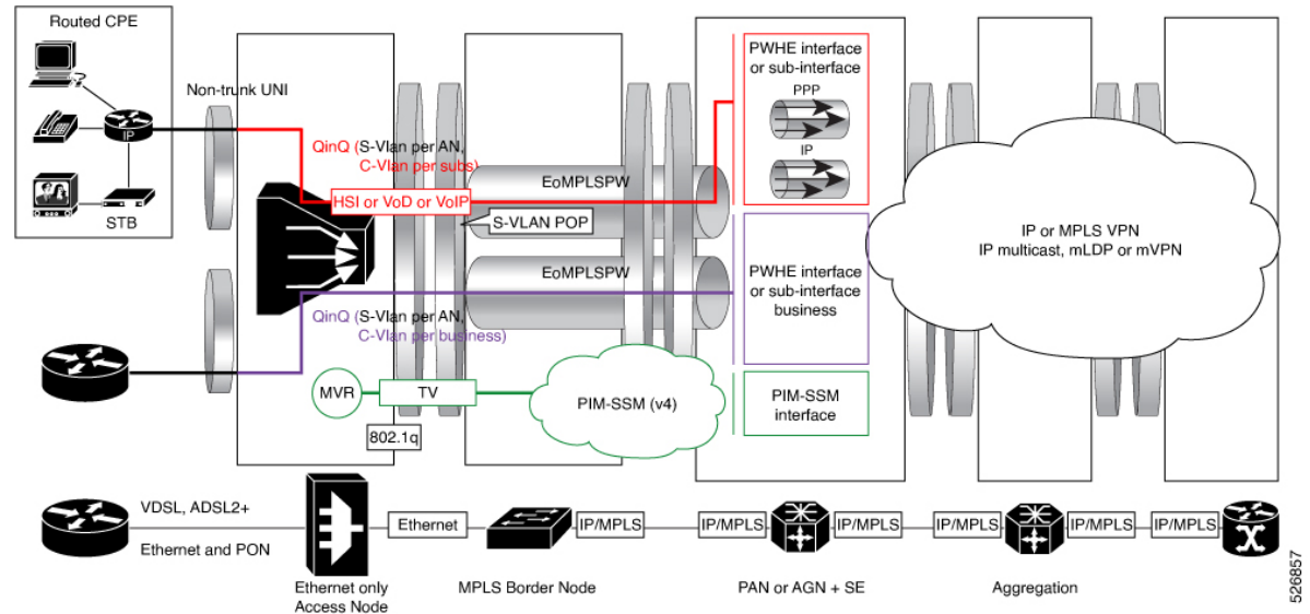
Figure 37: Deployment Model 2 for Residential and Business Subscribers on PWHE
