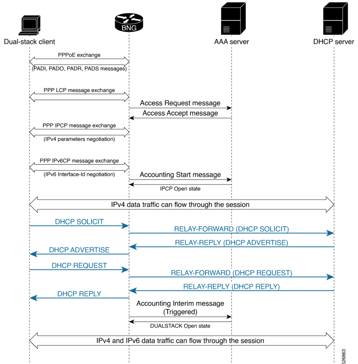
Figure 43: Call Flow of PPPoE Dual-Stack - DHCPv6-Based Address Assignment
