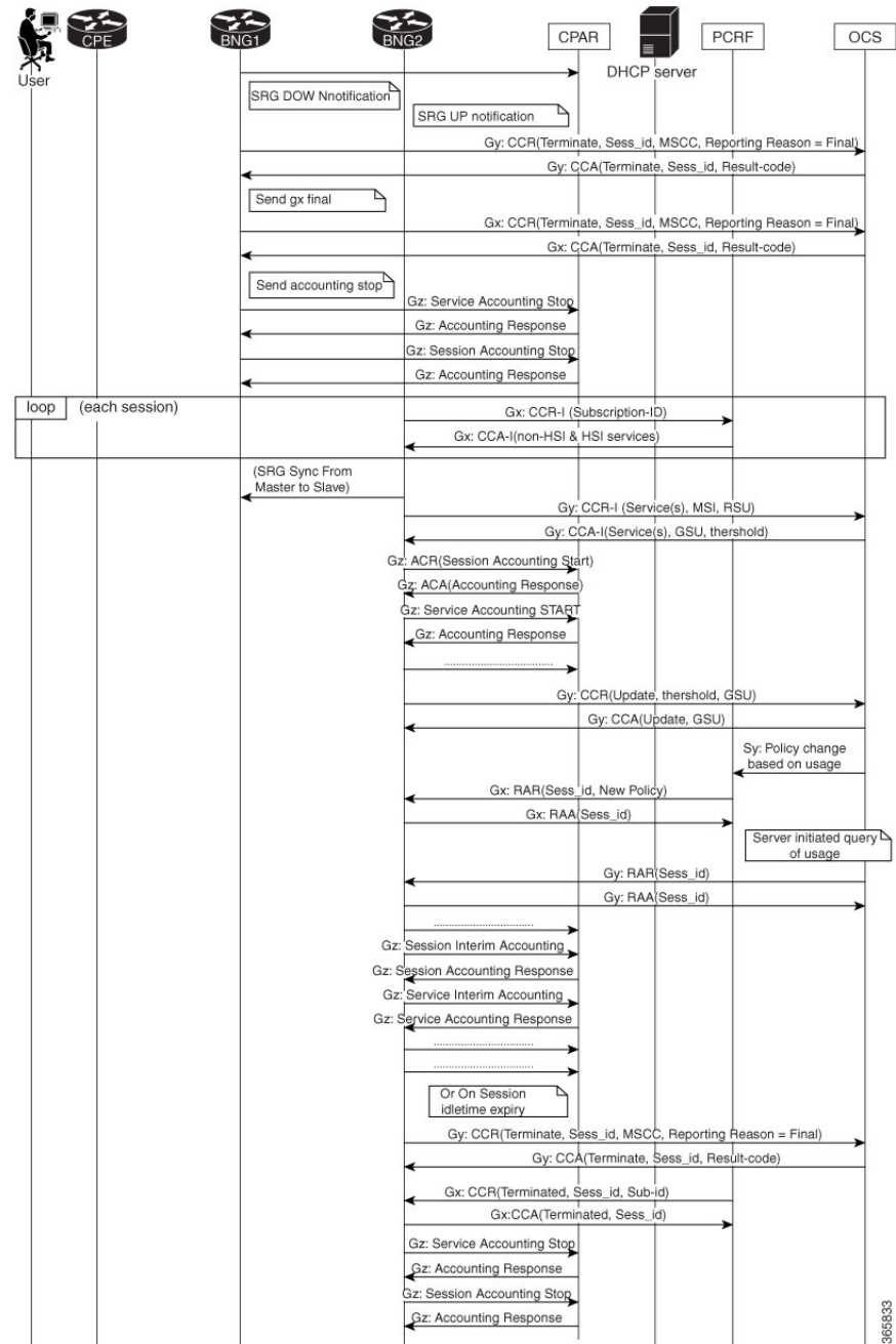
Figure 32: Call Flow of Subscriber Sessions During SRG Switch Over
