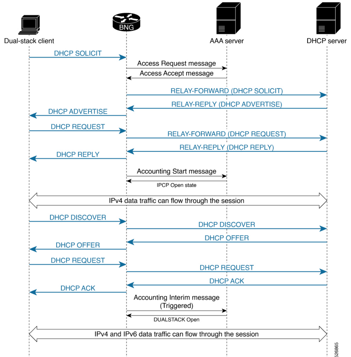
Figure 45: Call Flow of IPoE Dual-Stack - IPv6 Address-Family Starts First
