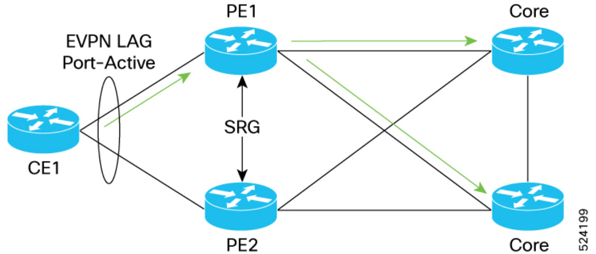
Figure 26: Topology for BNG with EVPN Port-Active with PE1 as the Primary Node
