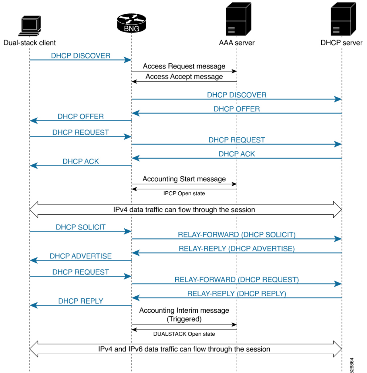
Figure 44: Call Flow of IPoE Dual-Stack - IPv4 Address-Family Starts First
