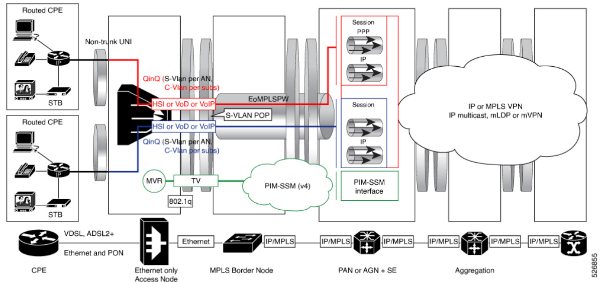
Figure 35: 1:1 deployment model for residential subscribers on PWHE
