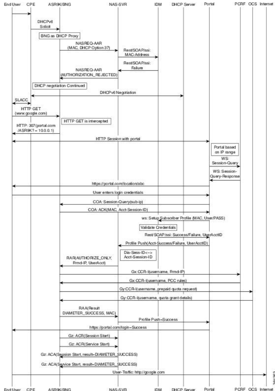
Figure 30: BNG DIAMETER Call Flow
