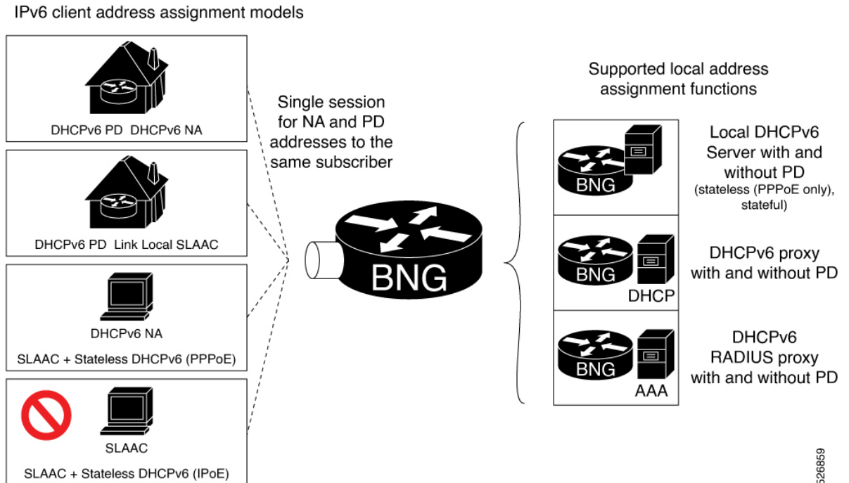
Figure 39: IPv6 Client Address Assignment Models
