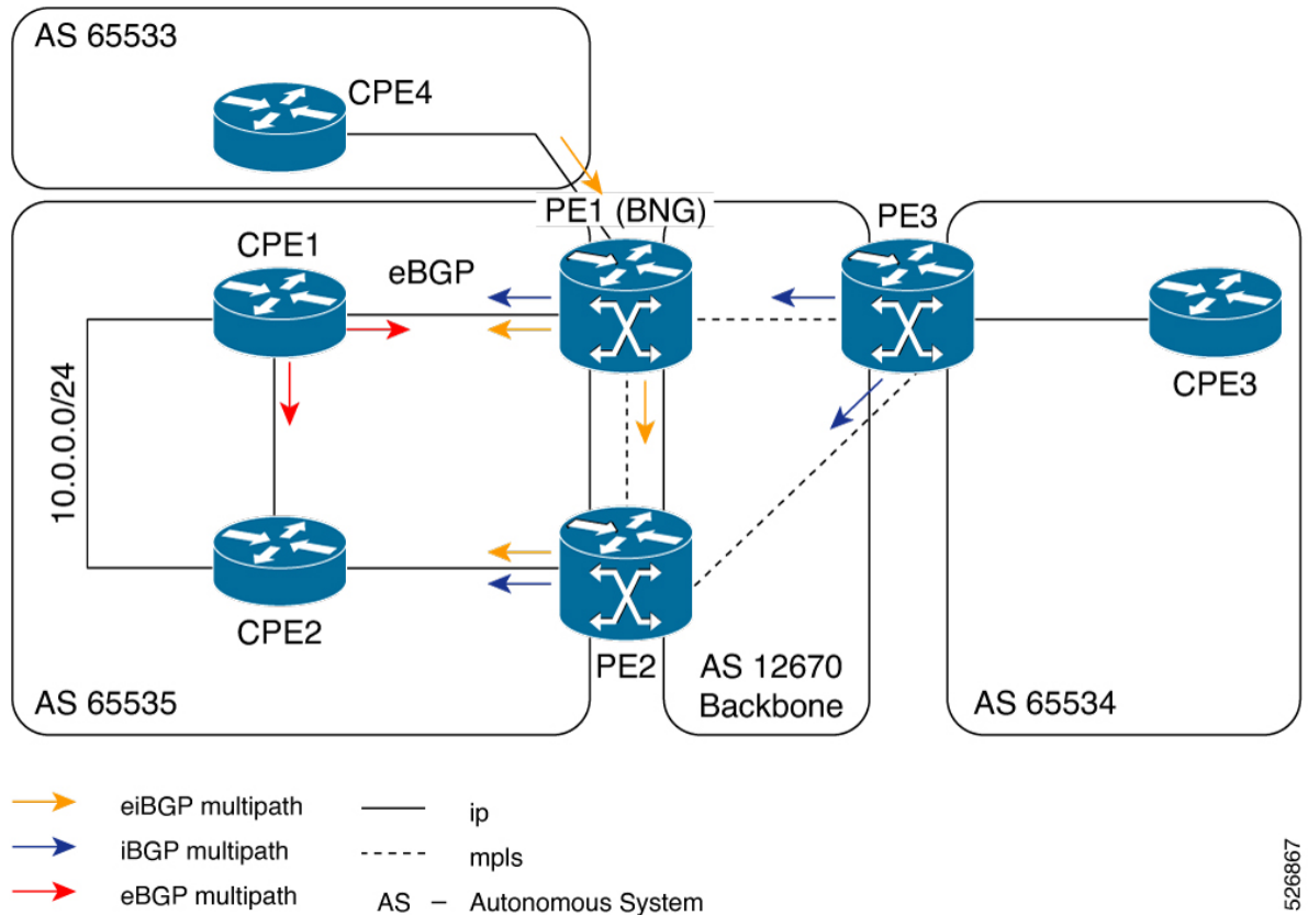
Figure 47: Sample topology for eBGP over PPPoE
