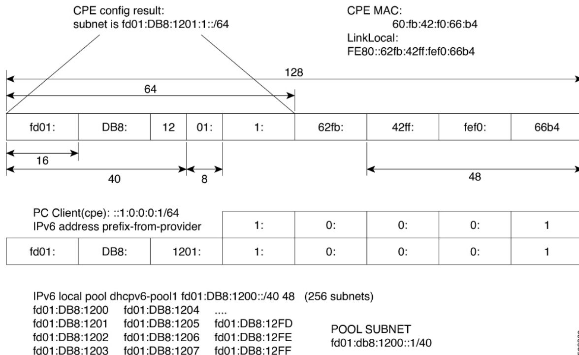
Figure 40: Sample IPv6 Address Mapping for Dual-Stack Subscriber
