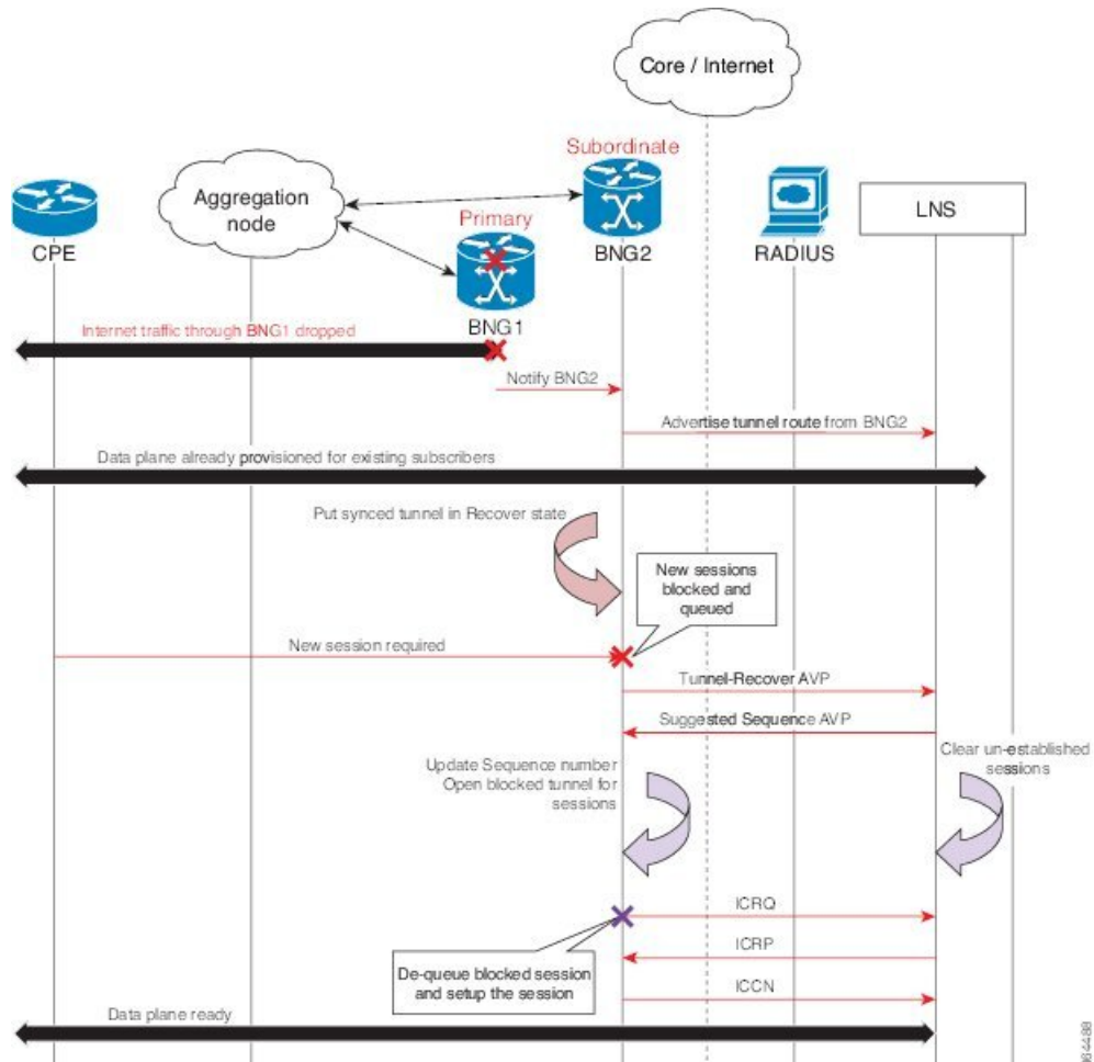
Figure 24: PPPoE-LAC Session Switchover
