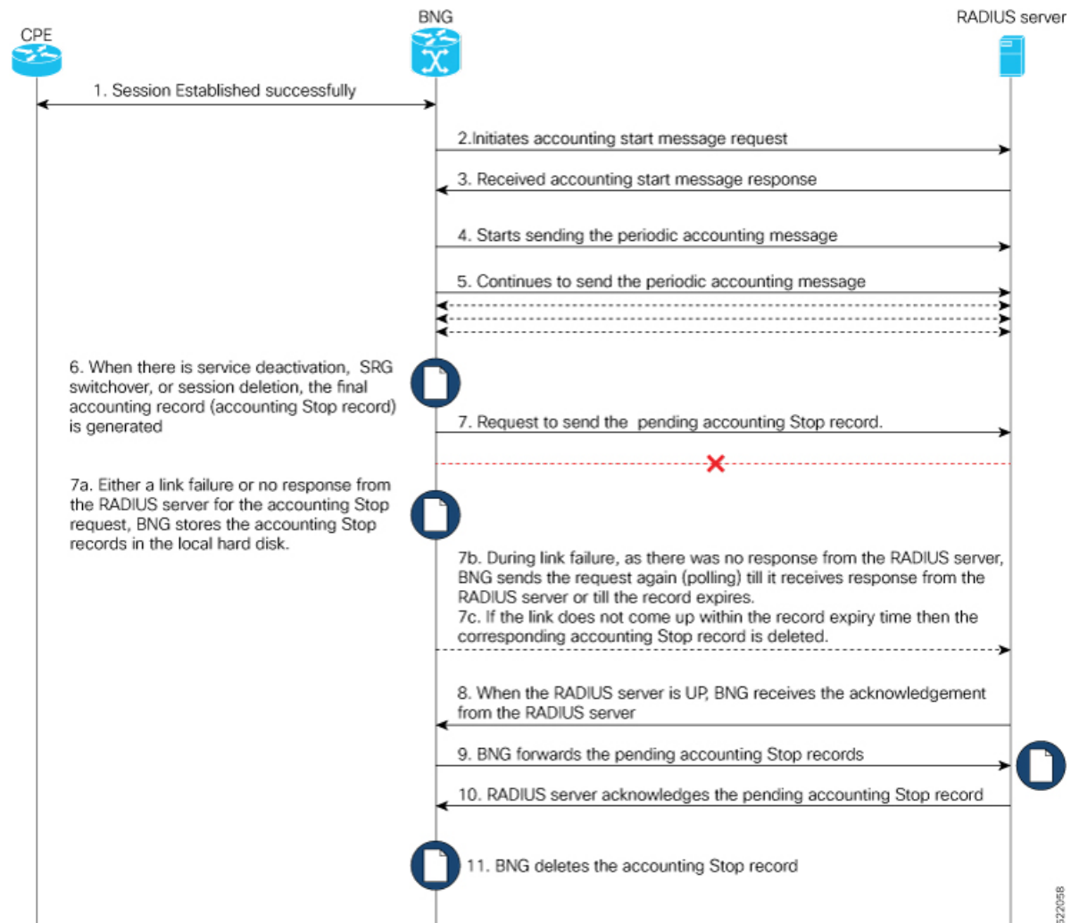
Figure 4: Sequence of events for forwarding accounting Stop record to the RADIUS Server
