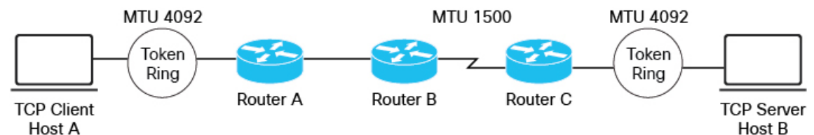
Figure 16: TCP MSS Adjustment
