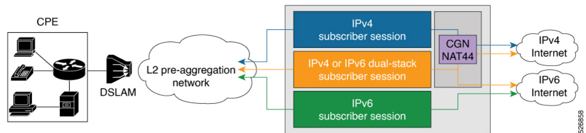
Figure 38: Deployment Model of Dual-Stack Subscriber Sessions
