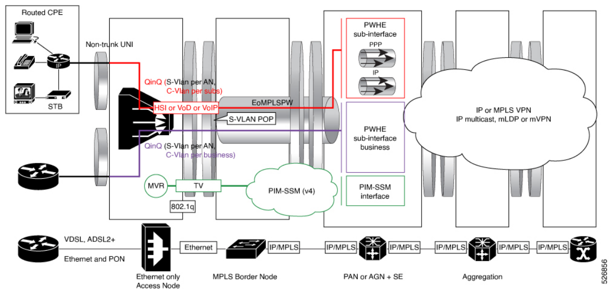
Figure 36: Deployment Model 1 for Residential and Business Subscribers on PWHE
