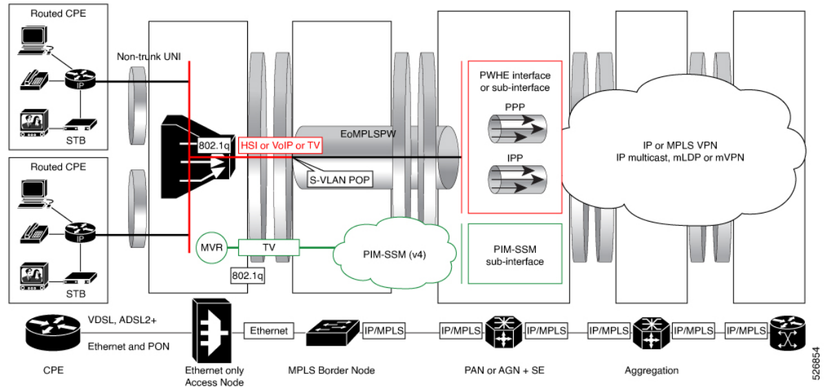
Figure 34: N:1 deployment model for residential subscribers on PWHE
