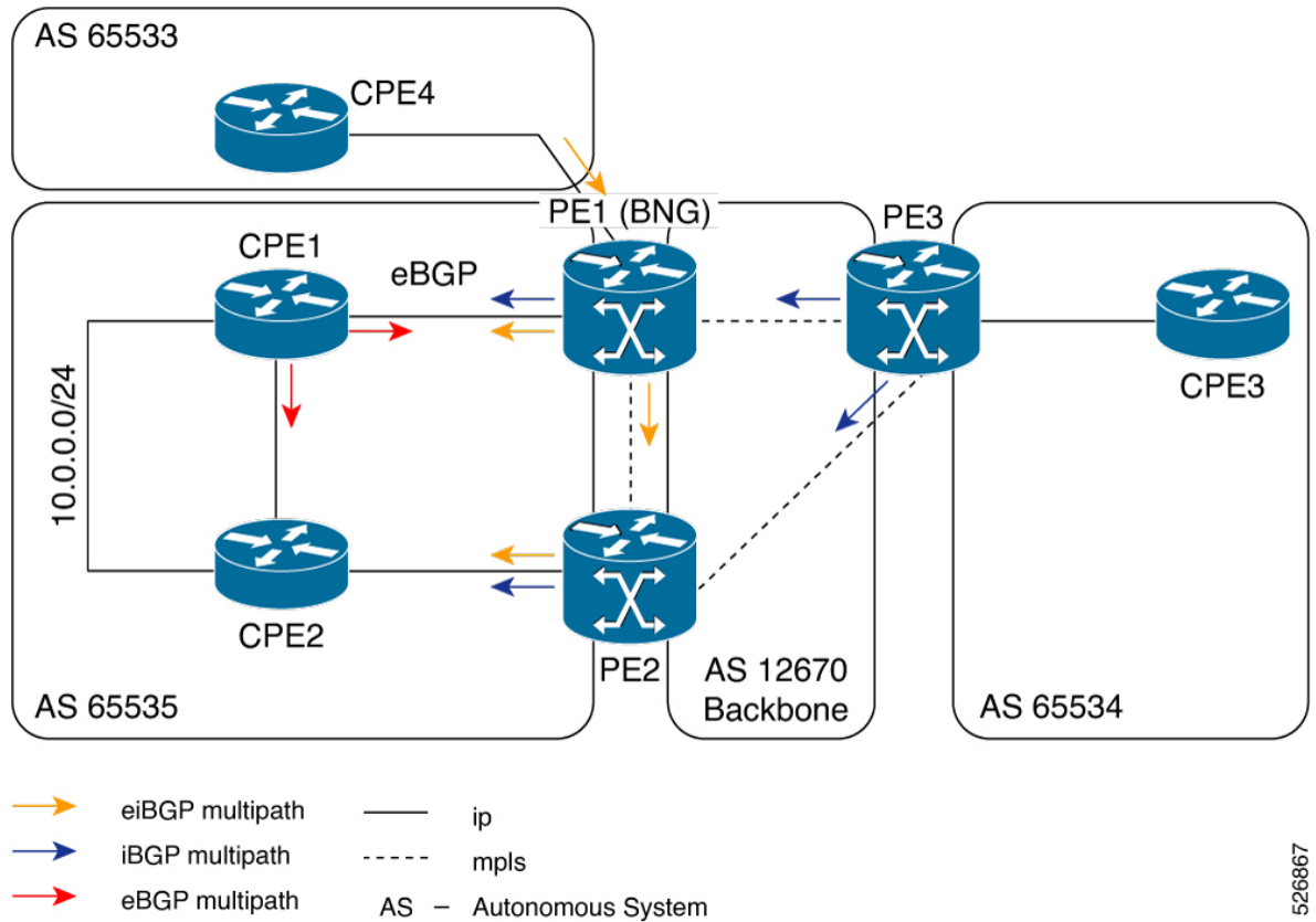
Figure 46: Sample topology for Dual-Stack
