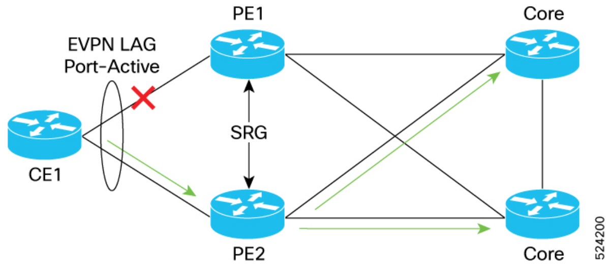
Figure 27: Topology for BNG with EVPN Port-Active with PE2 as the Primary Node
