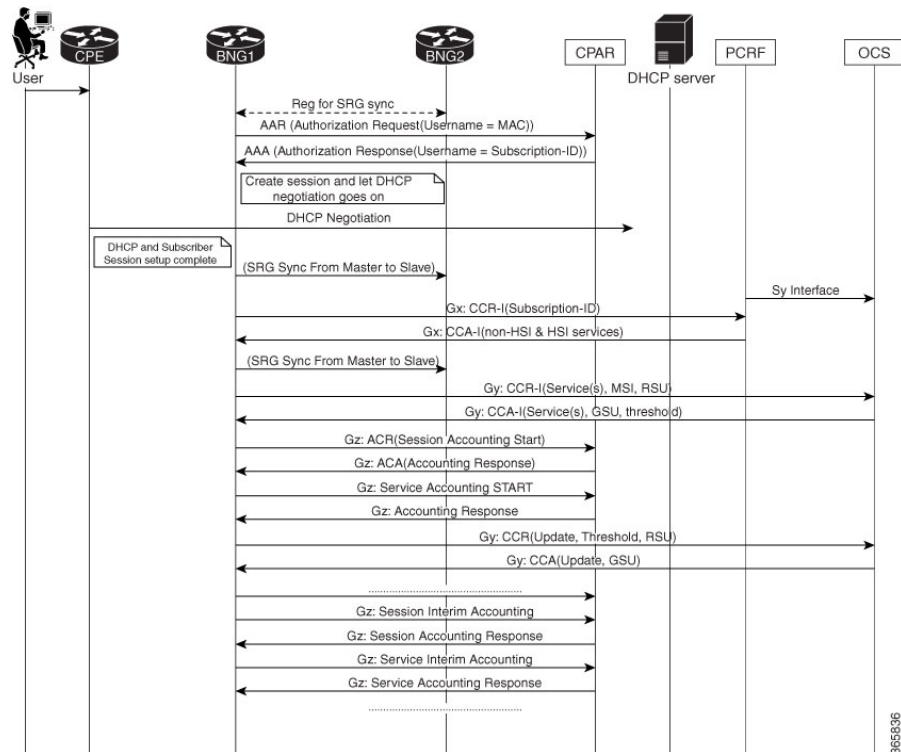
Figure 31: Call Flow of Subscriber Session Establishment With BNG DIAMETER-Geo Redundancy
