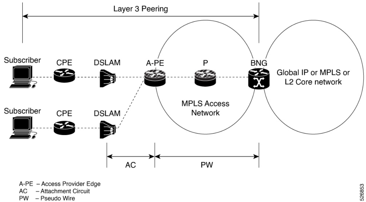
Figure 33: Sample Topology for BNG over Pseudowire Headend
