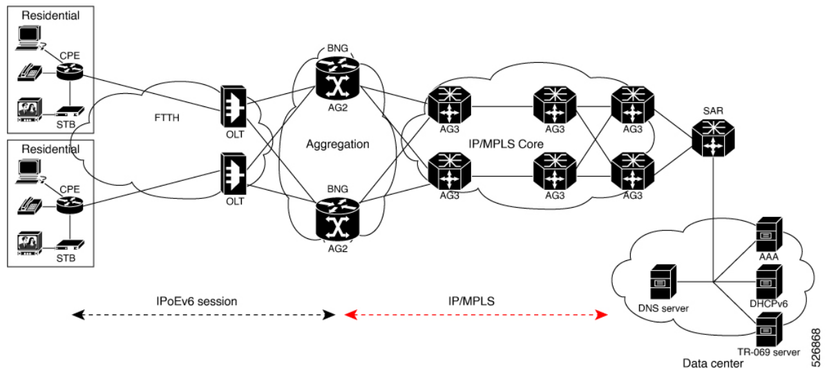
Figure 48: Sample Deployment Topology for Routed Subscriber Sessions
