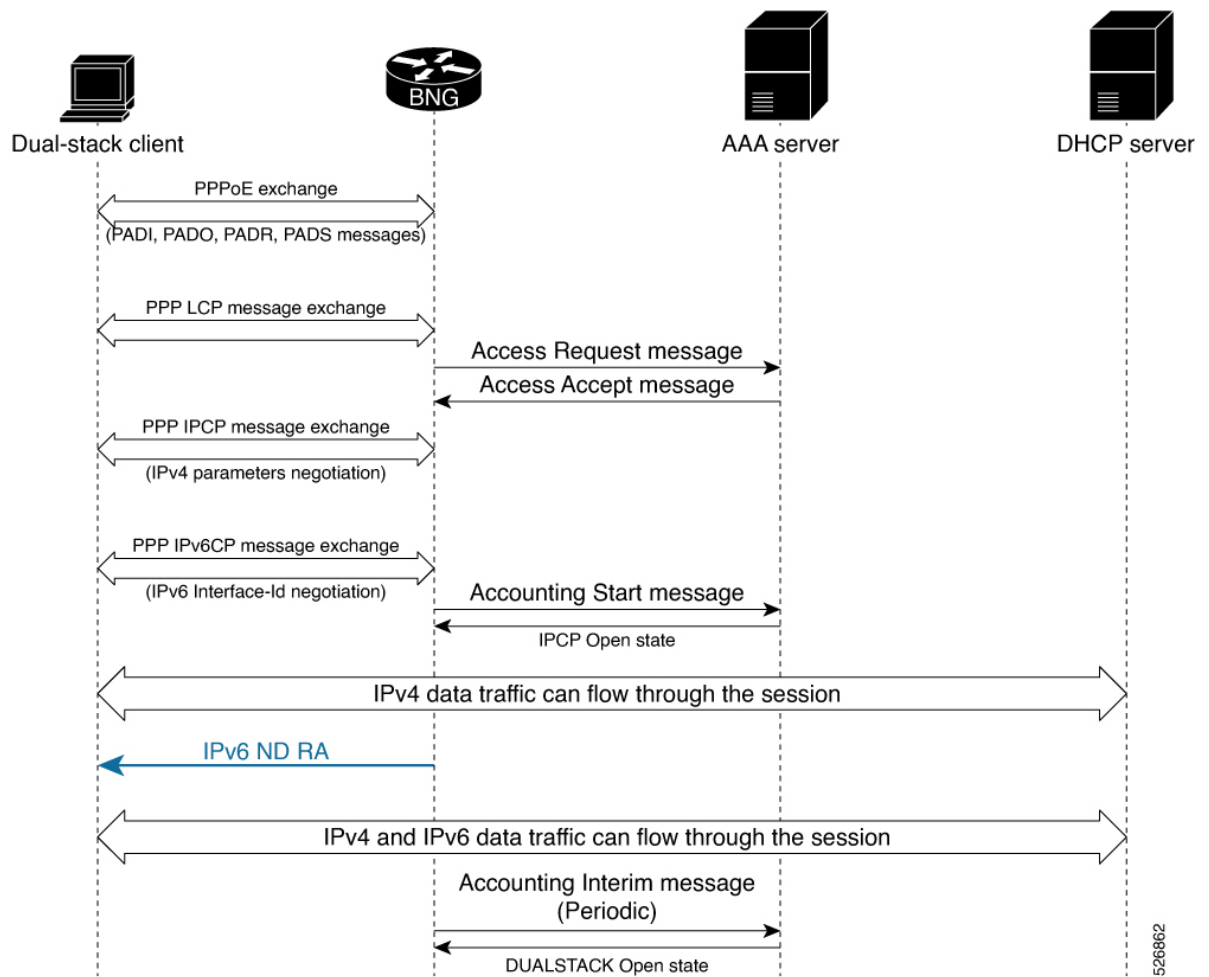
Figure 42: PPPoE Dual-Stack - SLAAC-Based Address Assignment
