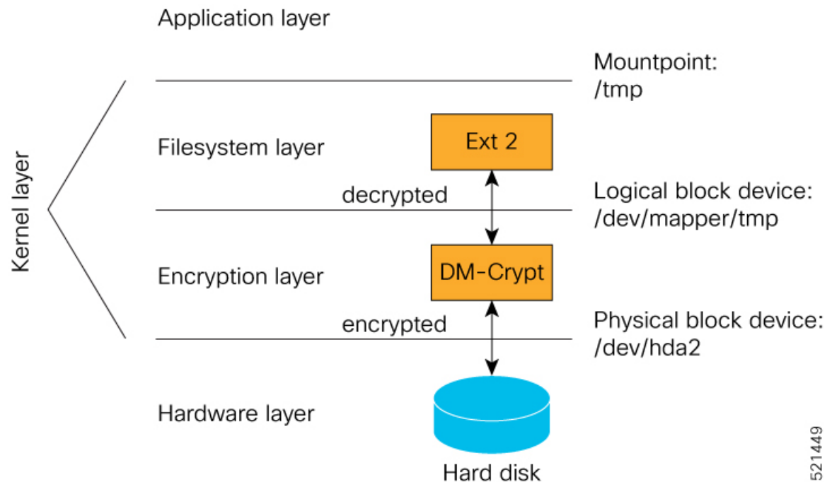
Figure 23: DM-Crypt Encryption
