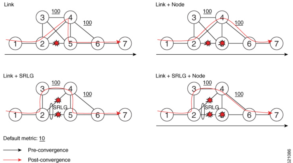
Figure 2: TI-LFA Protection Types
