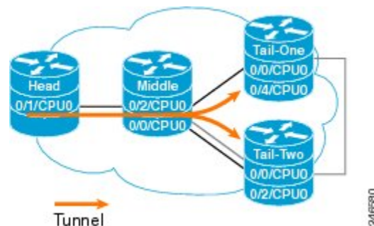
Figure 19: P2MP Topology
