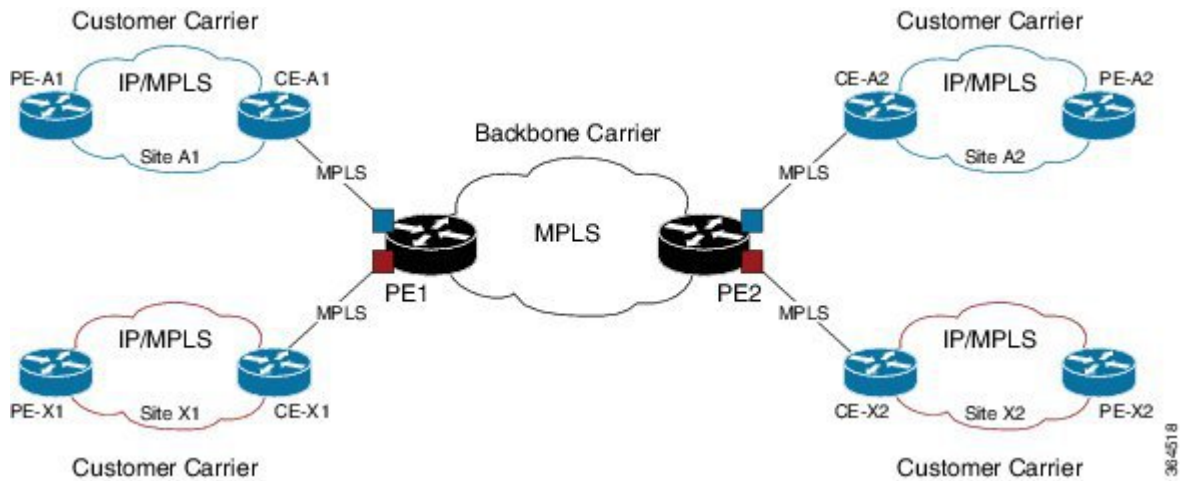
Figure 6: MPLS Carrier Supporting Carrier L3VPN
