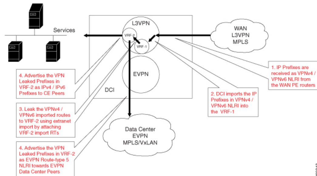
Figure 8: Advertise L3VPN Leaked Prefix
