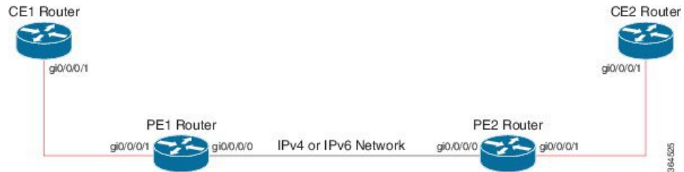
Figure 1: IP in IP tunnel network topology
