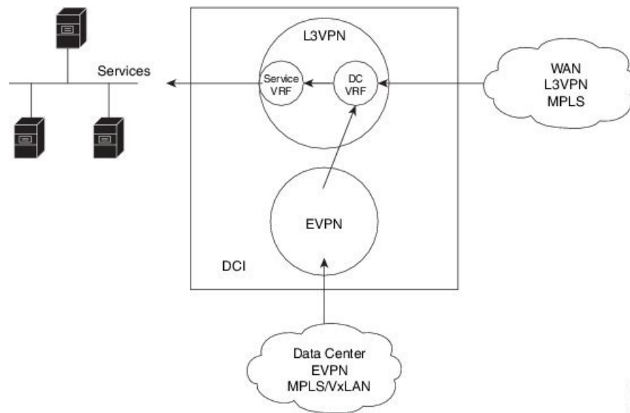
Figure 20: Leaking Routes to Service VRF from Data Center VRF
