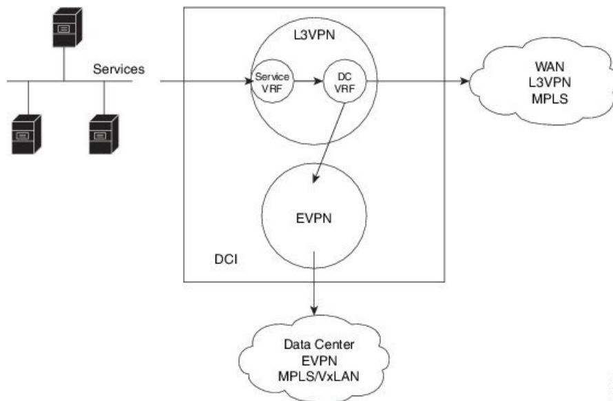
Figure 19: Leaking Routes from Service VRF to Data Center VRF
