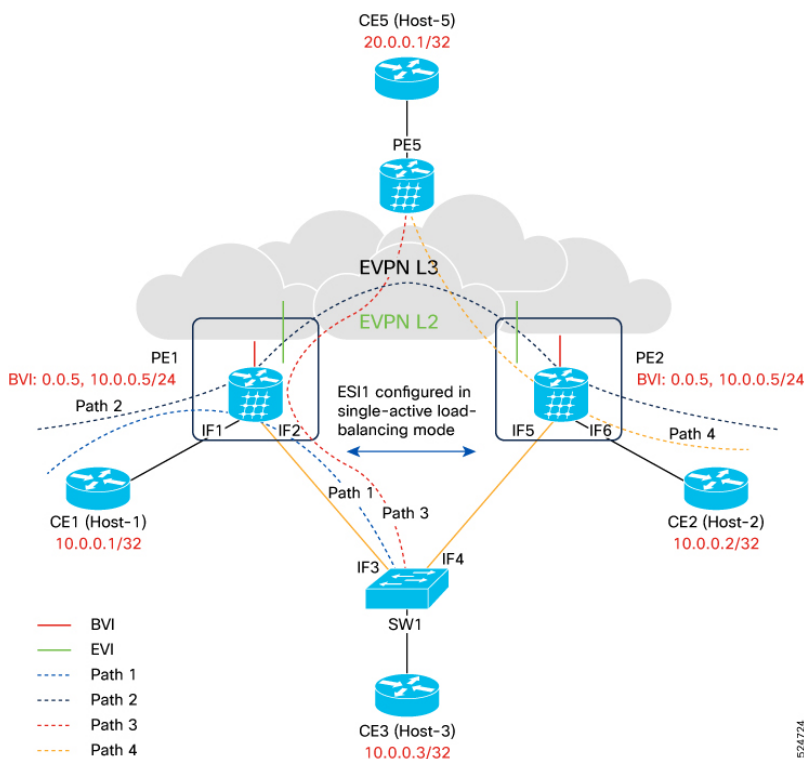
Figure 109: EVPN IRB single-homing network topology
