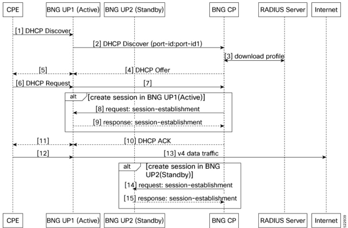
Figure 16: Subscriber Session Creation for Routed Subscribers
