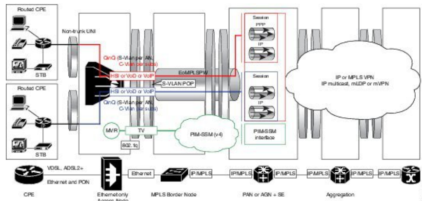
Figure 44: 1:1 deployment model for residential subscribers on PWHE
