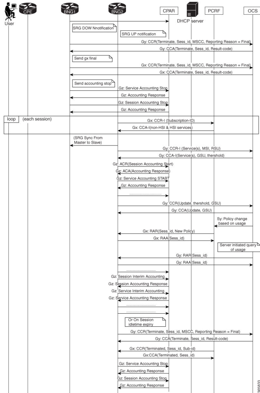
Figure 41: Call Flow of Subscriber Sessions During SRG Switch Over
