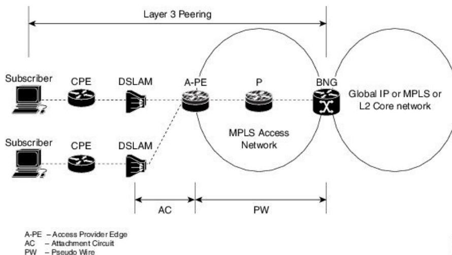
Figure 42: Sample Topology for BNG over Pseudowire Headend
