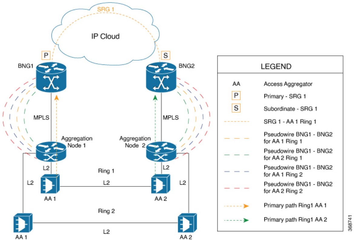
Figure 35: Sample Network Topology of SRG for PWHE Subscriber Sessions on BNG
