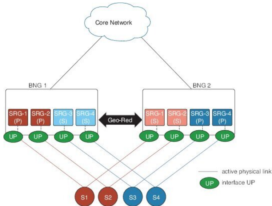
Figure 32: Active-active Session for BNG Geo Redundancy
