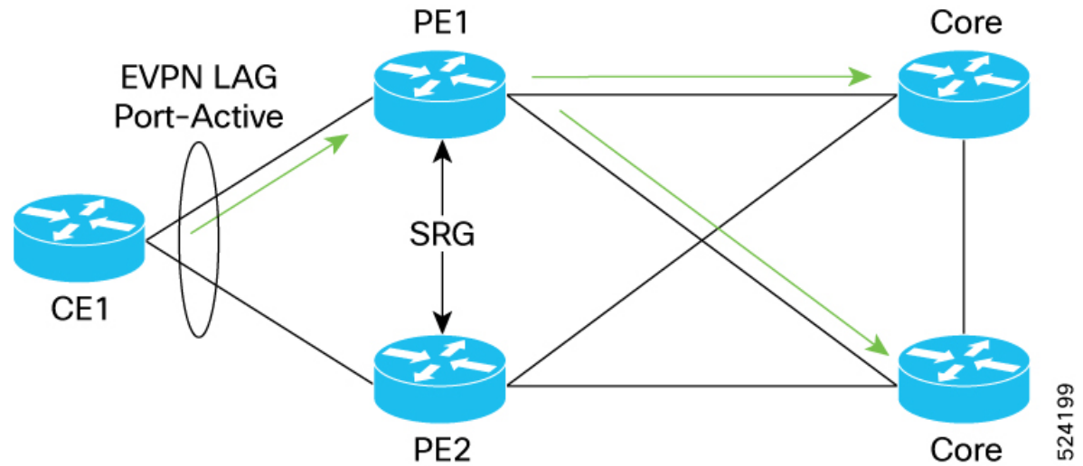
Figure 30: Topology for BNG with EVPN Port-Active with PE1 as the Primary Node
