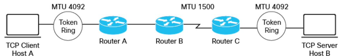
Figure 17: TCP MSS Adjustment
