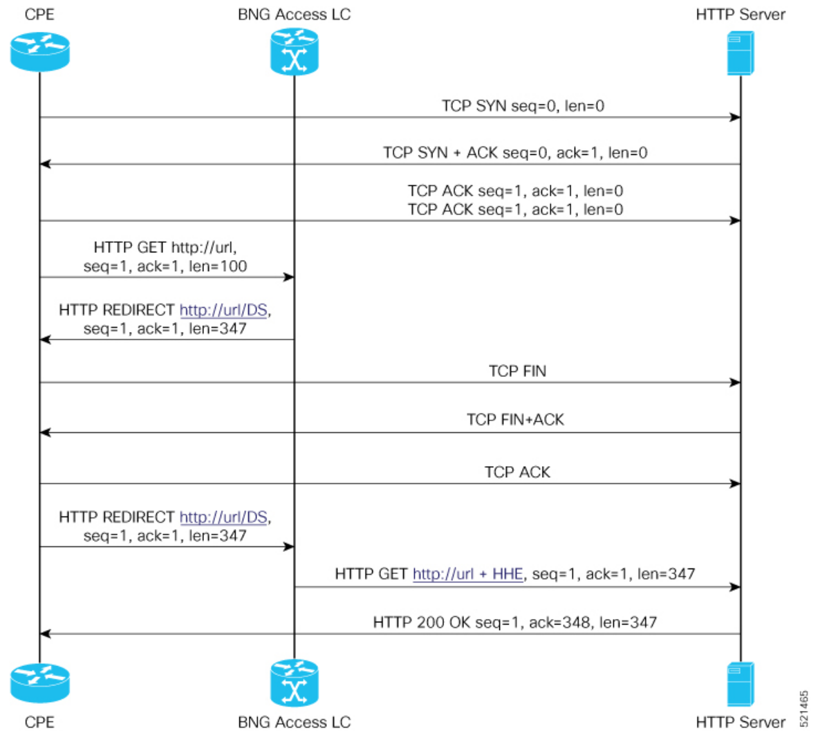
Figure 21: Sequence of events for HTTP Header Enrichment
