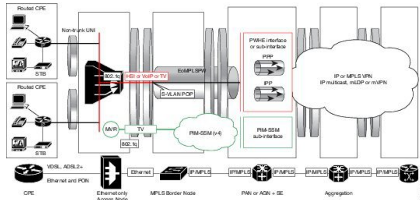
Figure 43: N:1 deployment model for residential subscribers on PWHE
