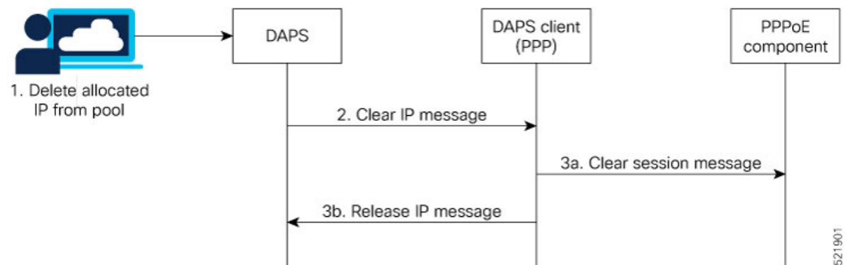
Figure 19: Call Flow of Dynamic Modification of DAPS Pool
