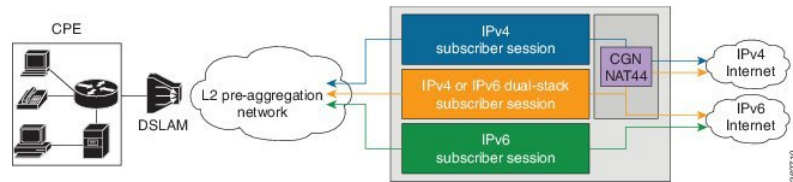
Figure 47: Deployment Model of Dual-Stack Subscriber Sessions
