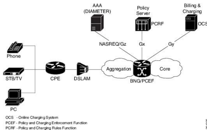
Figure 37: DIAMETER Interface in BNG
