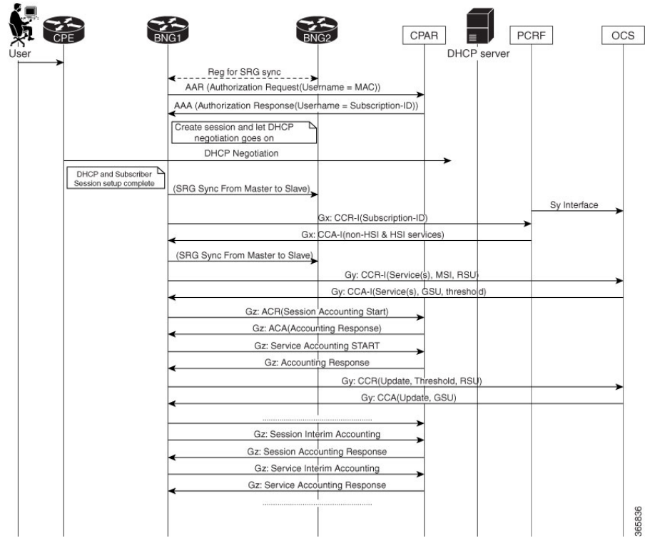
Figure 40: Call Flow of Subscriber Session Establishment With BNG DIAMETER-Geo Redundancy
