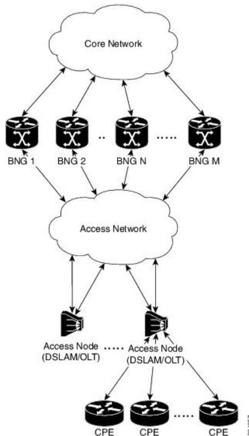
Figure 22: BNG Geo Redundancy Deployment Network Model
