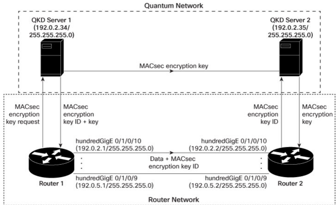
Figure 15: Point-to-Point MACsec Link Encryption using SKIP
