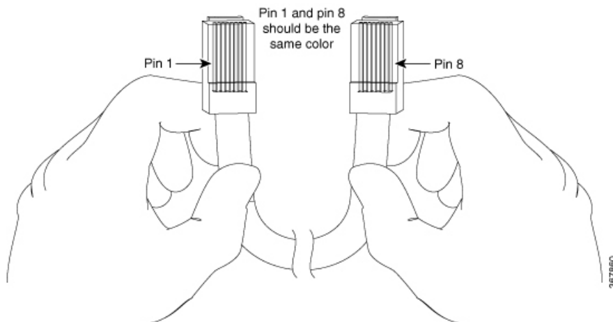
Figure 10: Identifying a Rollover Cable
