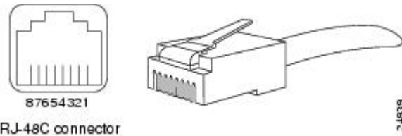
Figure 2: RJ-48C Connector
