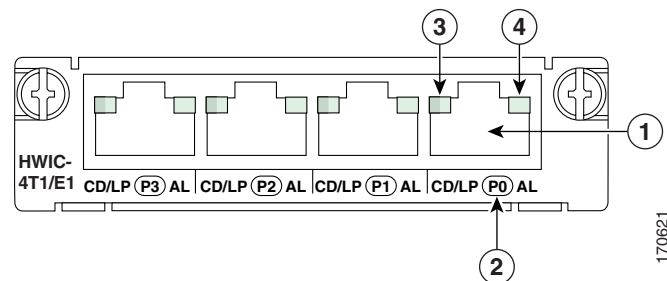
Figure 0-140 4-Port T1/E1 HWIC Front Panel
