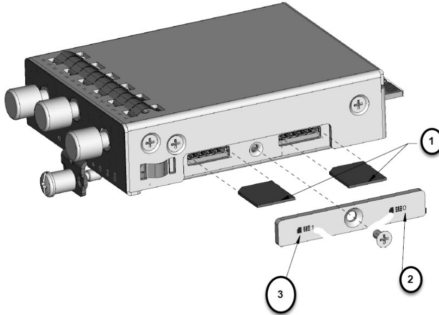
Figure 6: Sim Installation
