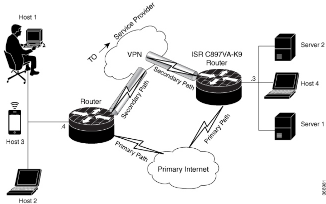
Figure 1: VPN-SIP Topology
