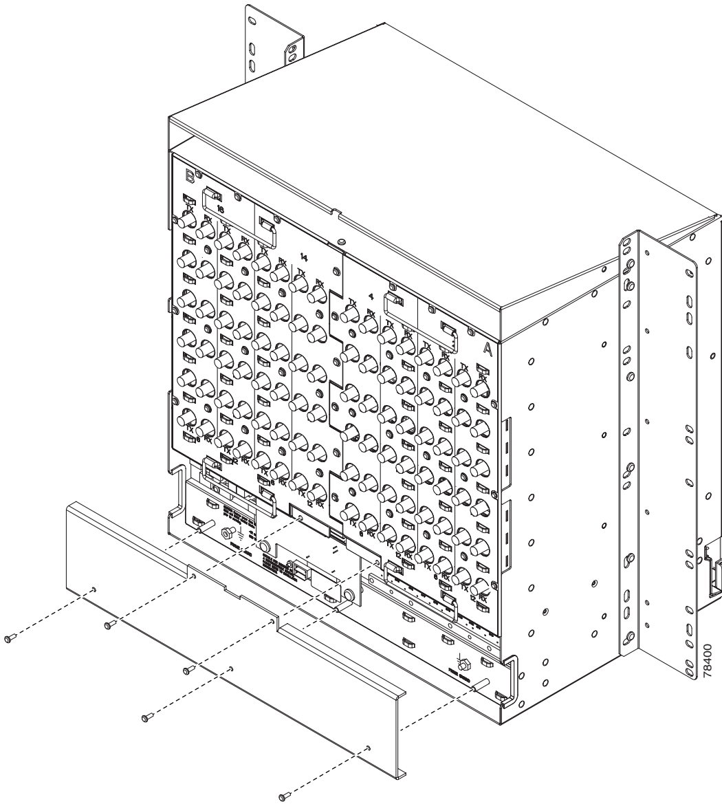
Figure 1 Attaching Plastic Lower Backplane Cover
