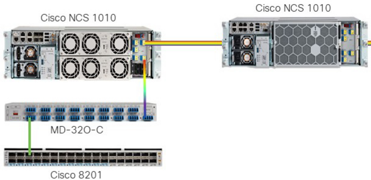
Figure 11: Point-to-point topology using NCS 1010 nodes
