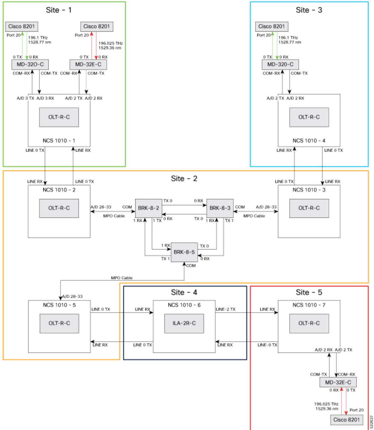
Figure 14: Wiring diagram for multi-degree topology
