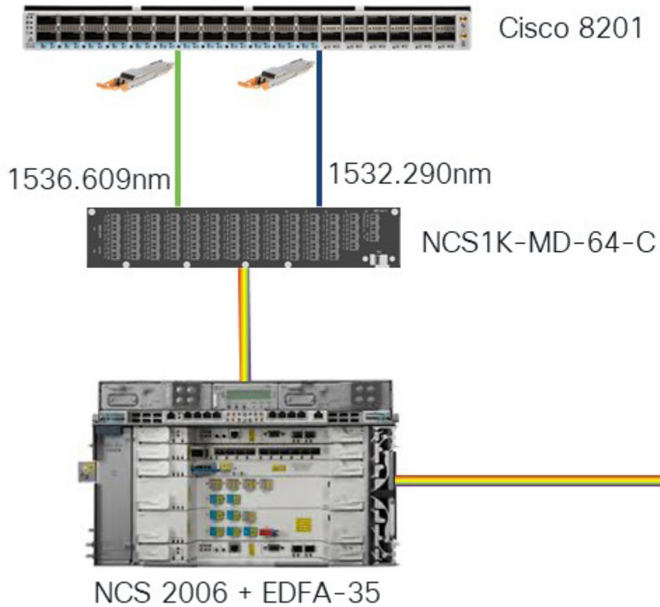
Figure 1: 400G-ZR P2P short haul applications with Cisco NCS 2006
