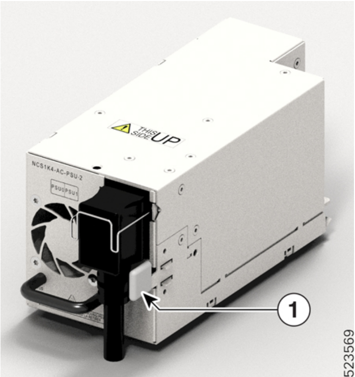
Figure 2: Locking Latch on the AC PSU
