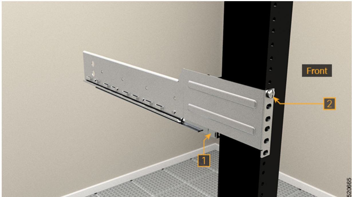
Figure 8: Two Post Slider Integration in the 19" Rack
