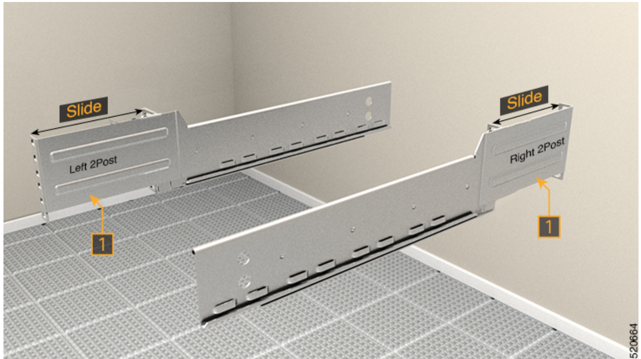
Figure 7: Two Post Slider Identification
