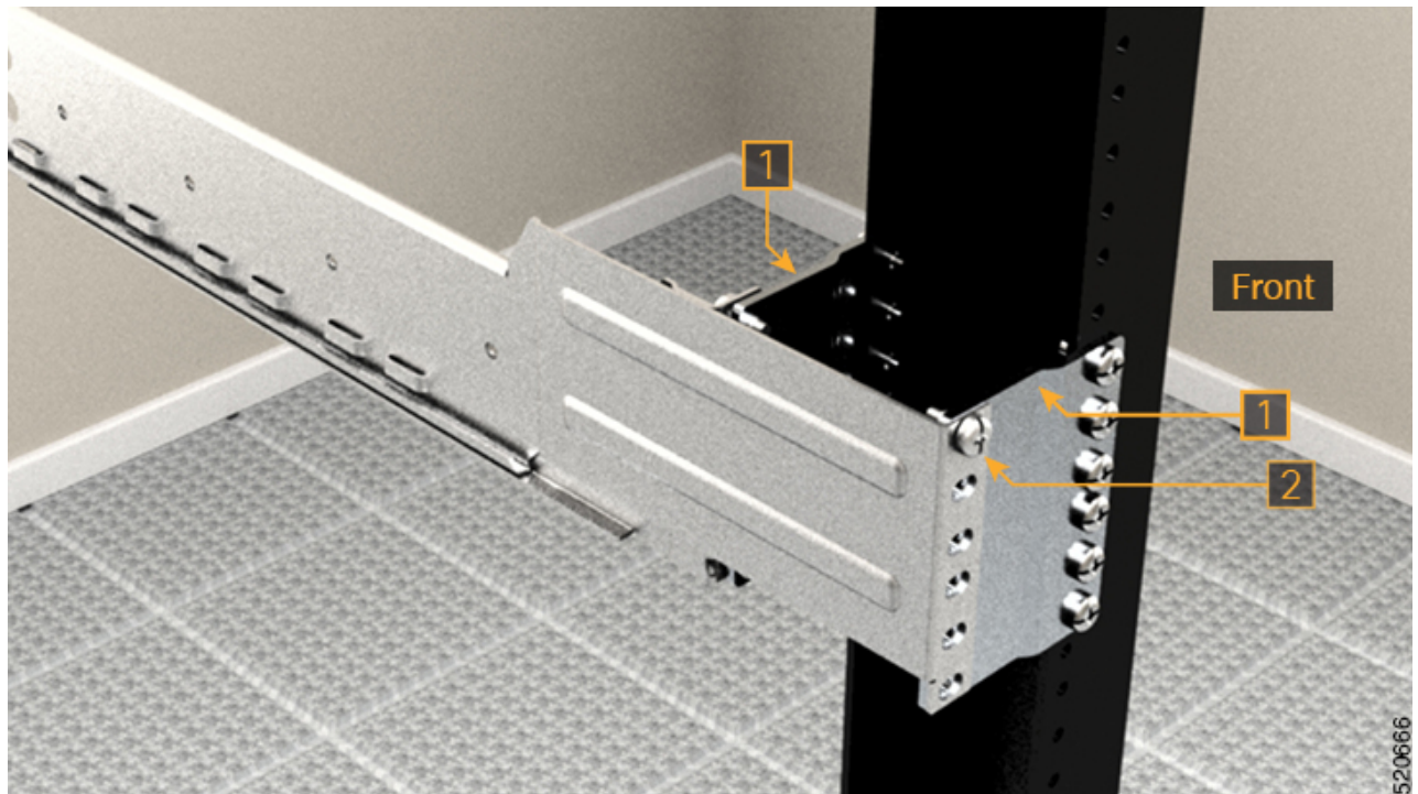
Figure 9: Two Post Slider Integration in the 23" Rack
