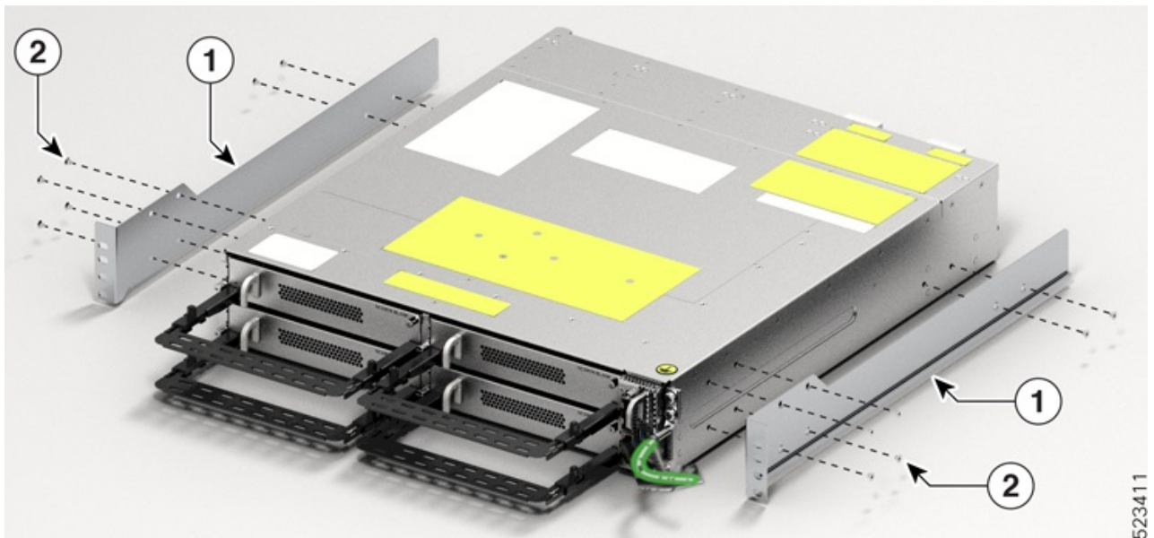
Figure 6: Fixing the Brackets
